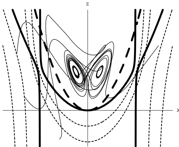
FIG. I-22 – Lorenz attractor enclosed by semipermeable surfaces of type (I.5-18) in case \gamma . The form of these surfaces for x^2 < \Leftrightarrow c_2 is a sink, what we cannot see in the figure, which is a projection. The bolded curve is given by the equality in expression (I.5-19). The thick dashed curved is the last parabola.
