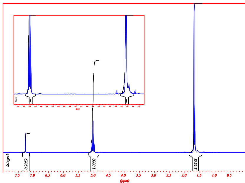
Figure 7 Spectre RMN 1 H du lactide sublimé
