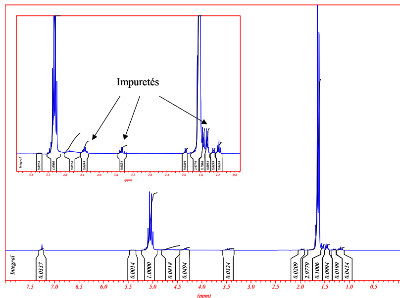
Figure 6 Spectre RMN 1 H du lactide commercial
