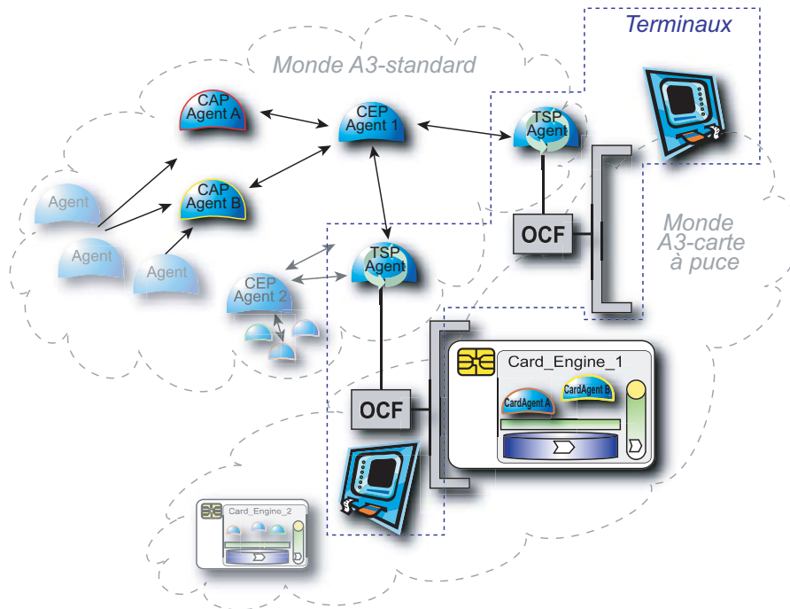
Figure 4.22 – Architecture A3/JavaCard.
