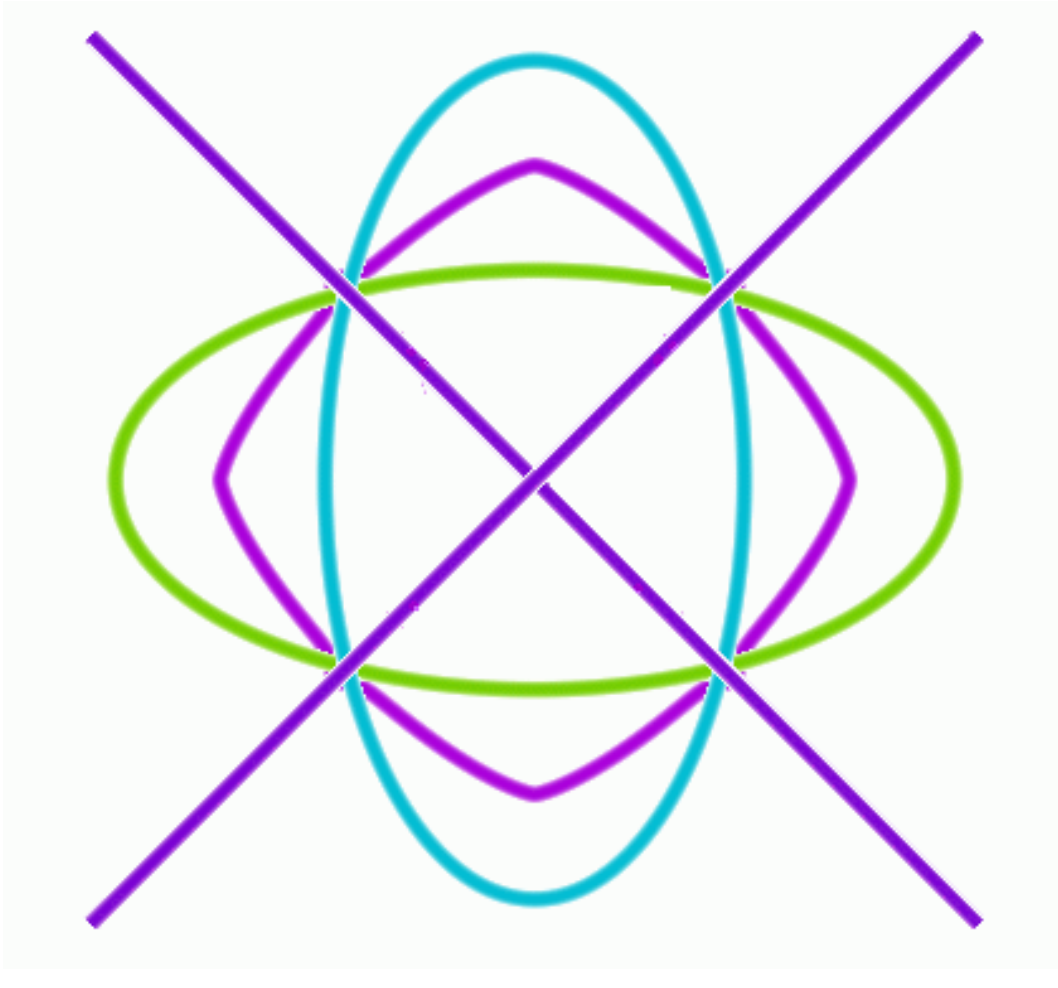
Figure 1.2.1: The relative position with respect to the bisector must be constant
