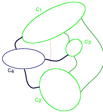
Figure 5.2.4: The new Delaunay graph after insertion of C_4 : the edges in plain thin lines remain, those in dashed lines disappear, and those in plain thick lines appear
