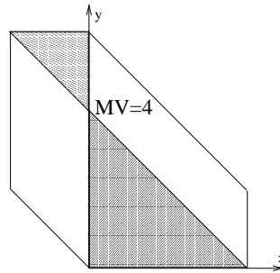
Figure 4.4.10: The mixed volume of f and n for ellipses and hyperbolas.
