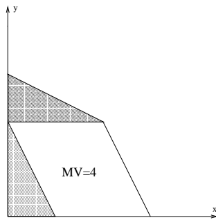
Figure 4.4.22: The mixed volume of f and f - d for parabolas.
