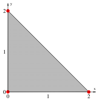
Figure 4.4.7: The Newton polytope of f for ellipses and hyperbolas.
