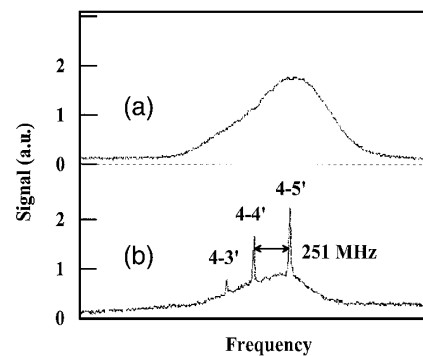
Fig. 2. Observation of the cold atoms in the storage cell. (a) Cooling light switched off: the Doppler effect broadens the hyperfine transitions of cesium atoms. (b) Cooling light switched on: the atoms are cooled and the hyperfine peaks are resolved.
