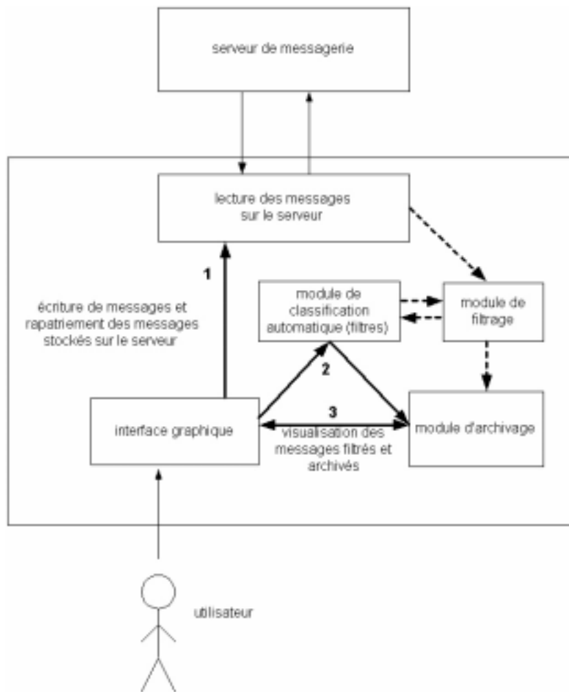
Figure 5.3 Architecture de Enaïm.
