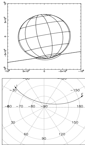
Figure 1: Raynaud et al. , Re-analysis of \beta Sco 1971 occultation data
