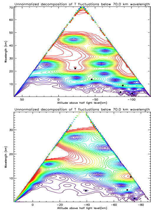
Figure 9: Raynaud et al. , Re-analysis of \beta Sco 1971 occultation data
