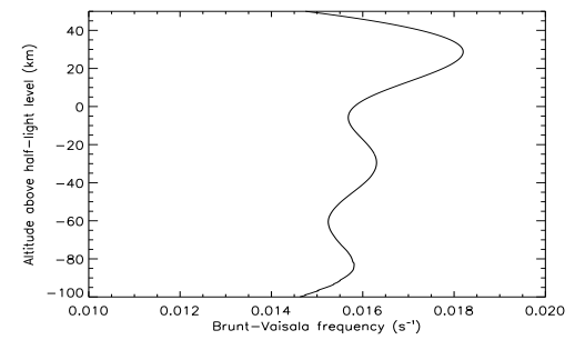
Figure 10: Raynaud et al. , Re-analysis of \beta Sco 1971 occultation data
