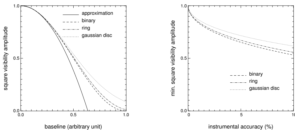
Fig. 4. Comparison between the exact visibility amplitude of an object and its second-order estimate. Different geometries have been assumed to show that little dependence is found: a symmetrical binary (dashes), a ring (dash-dot-dot), and a Gaussian disc (dots). The left panel displays the second-order estimate (solid line) and the exact visibilities of the different objects vs. the baseline. The right panel displays the visibility amplitude for which an observational difference can be made between the estimate and the exact value vs. the instrumental precision; it is the limit of validity for this estimate.
