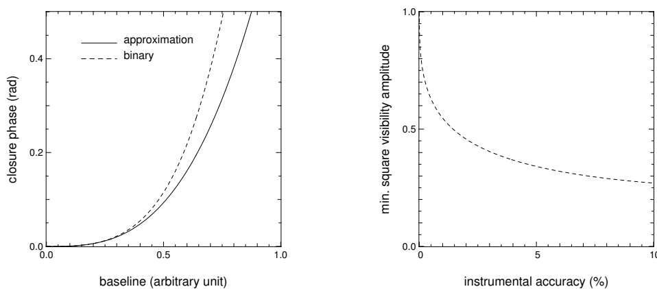
Fig. 5. Comparison between the exact closure phase of an asymmetrical binary ( \Delta\text{mag} = 1.2 ) and its third-order estimate. Left panel: closure phase vs. mean baseline. Right panel: minimum visibility for which no observational difference can be made between the estimate and the exact phase vs. instrument accuracy.
