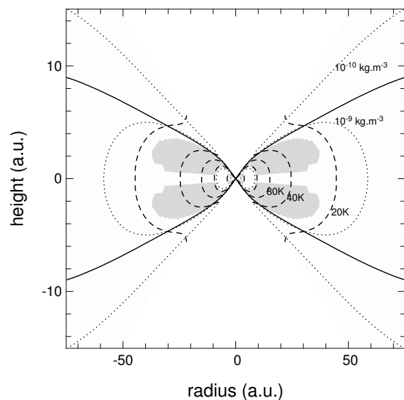
Fig. 1. Iso-contour maps of a T Tauri disk with \dot{M} = 10^{-5} M_\odot/\text{yr} . Dashed lines: lines of equal temperature; Dotted lines: lines of equal density; Solid line: limits of the optically thick region ( \tau = 1 ); Gray zone: zone of instability with respect to the convection.
