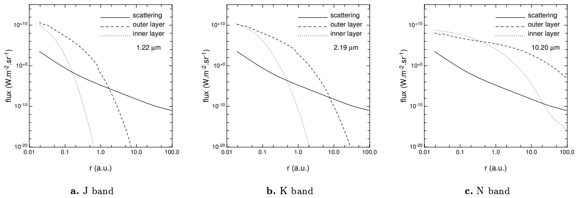
Fig. 7. Scattered light and thermal flux from a typical T Tauri disc (model 2) vs. the distance to the star. Left: J-band; middle: K-band; right: N-band. Solid lines: scattered light; dashed lines: thermal emission of the outer layer; dotted lines: thermal emission of the inner layer.
