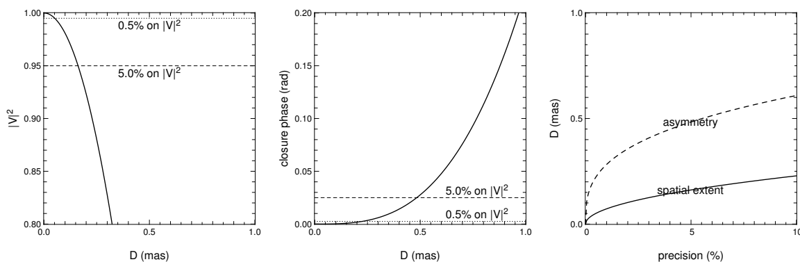
Fig. 3. Variation of the square visibility amplitude and closure phase with the angular size of a marginally resolved object for a 100 m baseline in K, and the detectability of these quantities. Left panel: square visibility amplitude vs. angular size; middle panel: closure phase vs. angular size; right panel: minimum object size needed to detect either the spatial extent or the asymmetry vs. the instrumental precision on |V|^2 . On the first left two view graphs the detection levels for 0.5% and 5% accuracy on |V|^2 measurements are displayed. We assumed a fairly asymmetric object with S = 0.5 , as well as \Delta\bar{\phi} = \Delta V .
