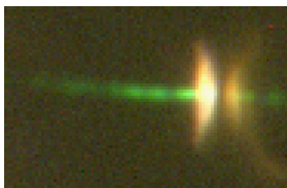
Figure 3: HH 30: Edge-on disc with a jet
