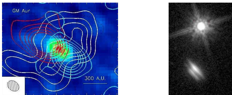
(c) Large-scale images. Left: radio map of GM Aur; right: IR image with AO of HK Tau (right)
