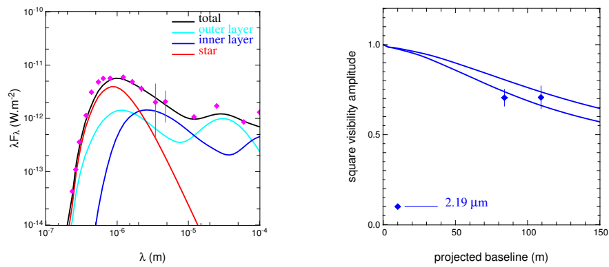
Figure 5: SU Aur: comparison between a two-layer flared disc model and observations. Left: SED; right: visibility vs. baseline.
