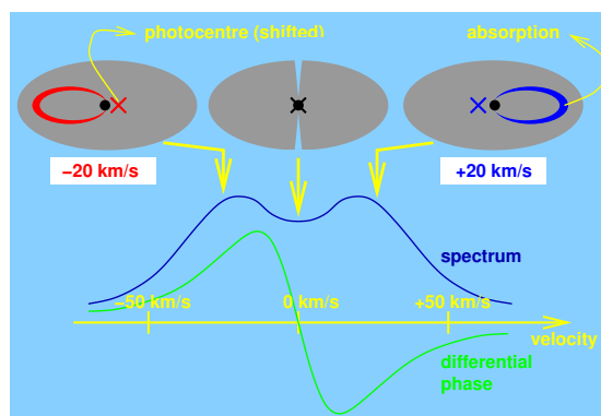
Figure 12: Measuring disc kinematics with the differential phase at high spectral resolution.
