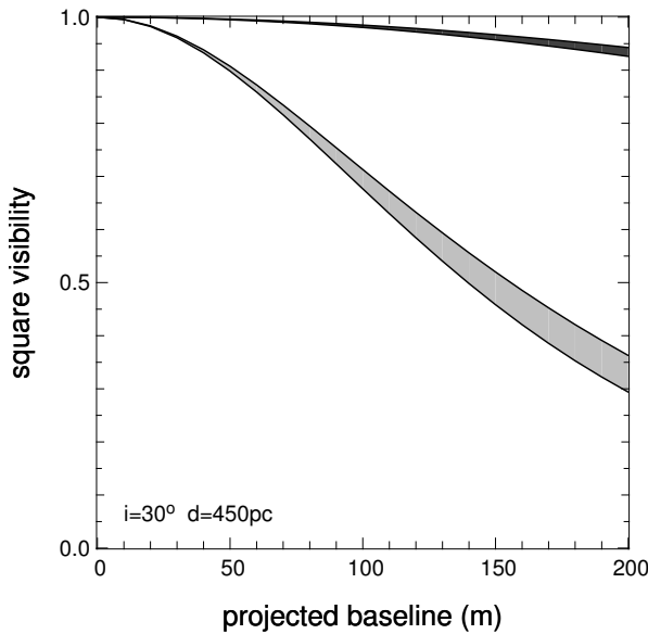
Fig. 8. Visibilities from a disk model as a function of the baseline. Gray : \dot{M} = 10^{-4} M_{\odot}/\text{yr} ; Black : \dot{M} = 10^{-6} M_{\odot}/\text{yr} . For a given baseline the visibility varies with the position angle; the domain between the minimum and maximum values is filled.
