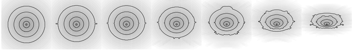
Fig. 10. Synthetic images of the thermal emission at 2.2 \mu\text{m} for different inclinations of the disk (from 0^\circ to 60^\circ by steps of 10^\circ ). \dot{M} = 10^{-6} M_\odot/\text{yr} . The field is 50 mas.
