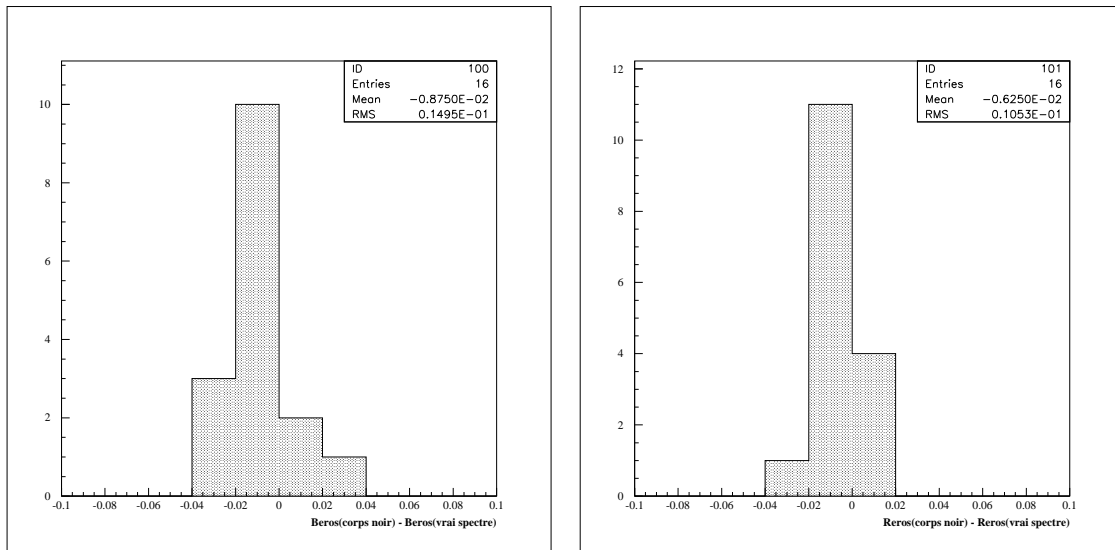
(a) m_B^{\text{Corps noir}} - m_B^{\text{Vrai spectre}}
