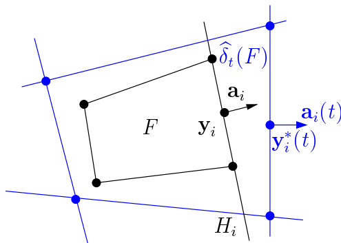
Figure 4.10: Over-approximation of \delta_t(F) .
