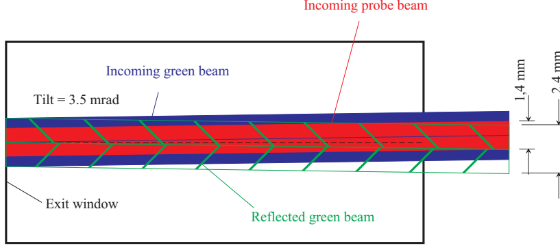
Figure 2.10: Reflection of the beams on the exit window, with a 3.5 mrad tilt (scheme not to scale).
