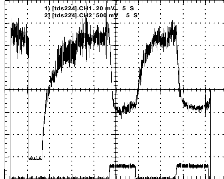
Figure 3.17: Trap signal (upper curve) and thermionic current (lower curve) vs time. The horizontal scale is 5 s per division. At t = 5 s, the magnetic field was turned off for 3 s in order to show the background level due to stray light.
