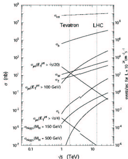
Figure 5.16.: Energy dependence of some proton-(anti-)proton cross-sections at the LHC and at the Tevatron. The discontinuity at \sqrt{s} = 4 \text{ TeV} is caused by the transition from p\bar{p} to pp , from [24].
