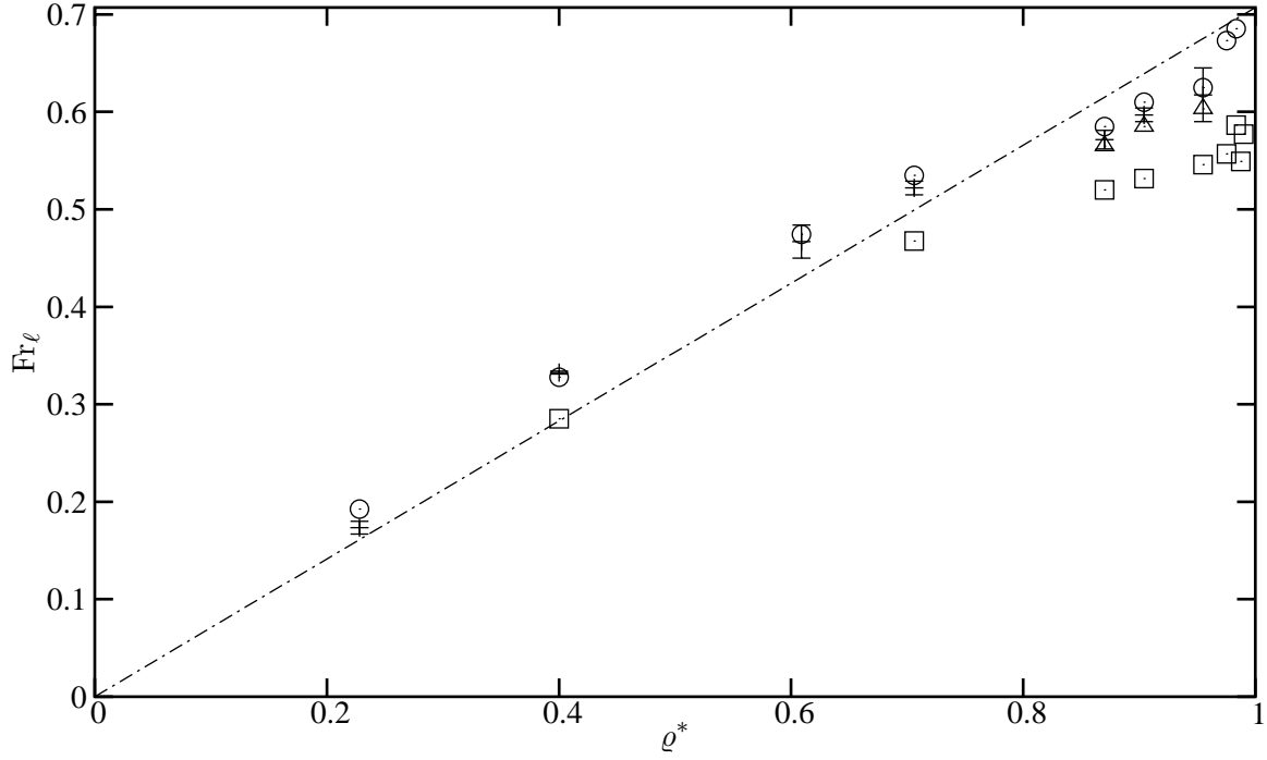
FIG. 15 – Froude number of the light front \text{Fr}_\ell versus \varrho^* in experiments and numerical simulations for both viscosity models. +, experimental values; \circ , numerical simulations with constant dynamic viscosity model ( \Lambda = 1 ) and \text{Re} = \varrho_{\text{air}} h \sqrt{\alpha g h} / \mu_{\text{air}} ; \square , numerical simulations with constant kinematic viscosity model ( \Lambda = 1 + \alpha \Phi ) and \text{Re} = \varrho_{\text{air}} h \sqrt{\alpha g h} / \mu_{\text{air}} ; \triangle , numerical simulations with constant dynamic viscosity model ( \Lambda = 1 ) and \text{Re} = \varrho_{\text{He}} h \sqrt{\alpha g h} / \mu_{\text{He}} . Error bars for the experimental values represent the discrepancies found between Figures 2 and 6 in the article by Gröbelbauer et al. [24] – · · ·, joins the theoretical limits for \varrho^* = 0 and \varrho^* = 1 according to \text{Fr}_\ell = \frac{\varrho^*}{\sqrt{2}} .
