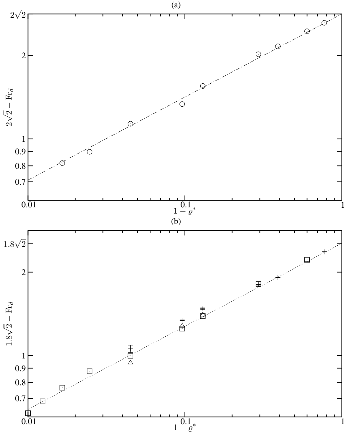
FIG. 17 – Correlation law between Froude number of the dense front Fr_d and 1 - \varrho^* . (a), \circ , numerical simulations with constant dynamic viscosity model ( \Lambda = 1 ) and Re = \varrho_{air} h \sqrt{\alpha g h} / \mu_{air} ; - \cdot - , 2\sqrt{2} (1 - (1 - \varrho^*)^{0.3}) . (b), + , experimental values; \square , numerical simulations with constant kinematic viscosity model ( \Lambda = 1 + \alpha \Phi ) and Re = \varrho_{air} h \sqrt{\alpha g h} / \mu_{air} ; \triangle , numerical simulations with constant dynamic viscosity model ( \Lambda = 1 ) and Re = \varrho_{He} h \sqrt{\alpha g h} / \mu_{He} . - - - , 1.8\sqrt{2} (1 - (1 - \varrho^*)^{0.3}) .
