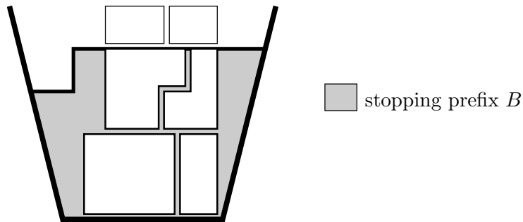
Figure 3.13: Lemma IV-2.1
