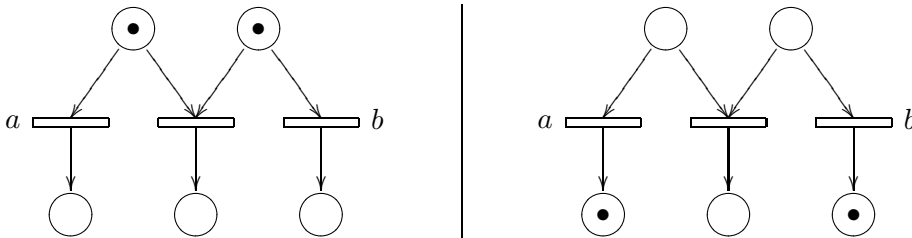
Figure 1.3: Transitions a and b are concurrent.
