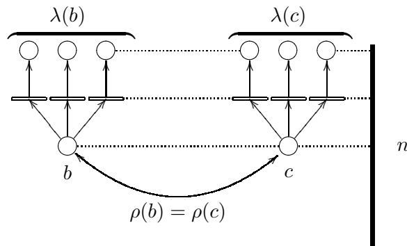
Figure 5.2: Non homogeneous Markov chain.
