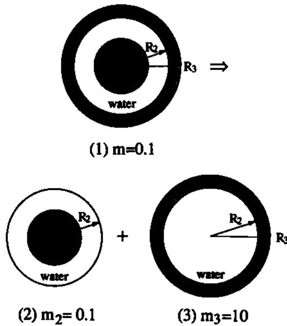
Fig. 2.12. [Hu and Joseph, 1989a] Diagram showing how three-layer core-annular flow could be understood from the composition of two two-layer flows.
