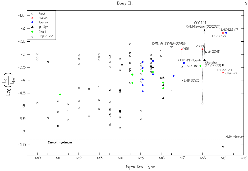
Fig. 3. Distribution of X-ray luminosity of M dwarfs as a function of spectral type. The open squares represent the values obtained for field M-dwarfs. The circles, diamonds, triangles up and down denote young objects in star-forming regions. The stars represent the flaring objects at their maximum with the corresponding value or upper limit on the quiescent emission. While DENIS J155601-233809 seems to have a normal X-ray luminosity in comparison with other M6~M7 dwarfs, GY 141 shows a strong variability between the Chandra and XMM-Newton observations. To avoid confusion, the spectral types of some objects have been shifted by 0.1 subclass. Values are from Martín & Bouy (2002) and references therein, except the quiescent value for VB 10, which is from Fleming et al. (2003).
