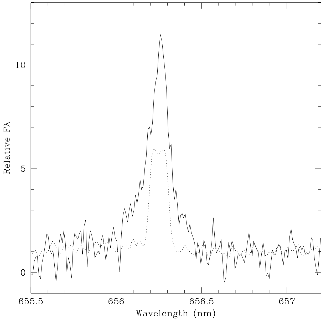
Figure 3.9 HRES spectra of DENIS-P J185950.9-370632 (solid line) and Gl 406 (dotted line) in the H \alpha region. Gl 406 is a typical chromospherically active M6 dwarf. DENIS-P J185950.9-370632 has a much broader and asymmetric emission line, indicating that it is probably an accretor.
