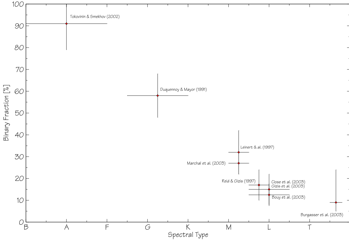
Figure 1.13 Binary frequency as a function of spectral type. Comparison of results obtained by several authors. Although it is not strictly rigorous to compare these values that were obtained under different conditions, there seems to be a trend for decreasing binary fraction with increasing spectral type. See also Figure 1 of the Introduction (page 14).
