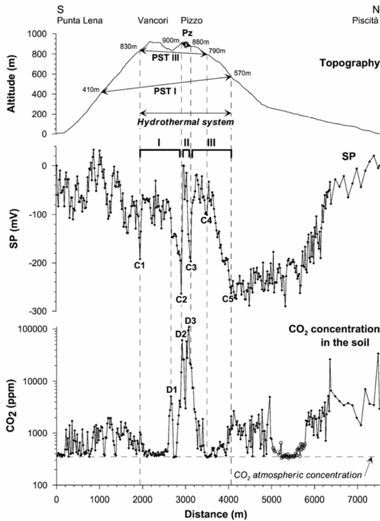
Fig. 5. Comparison between SP and \text{CO}_2 soil concentration along the Punta Lena–Piscità profile. Open circles: zone covered with concrete along the tourist trail. Other legends: same as Fig. 4.
