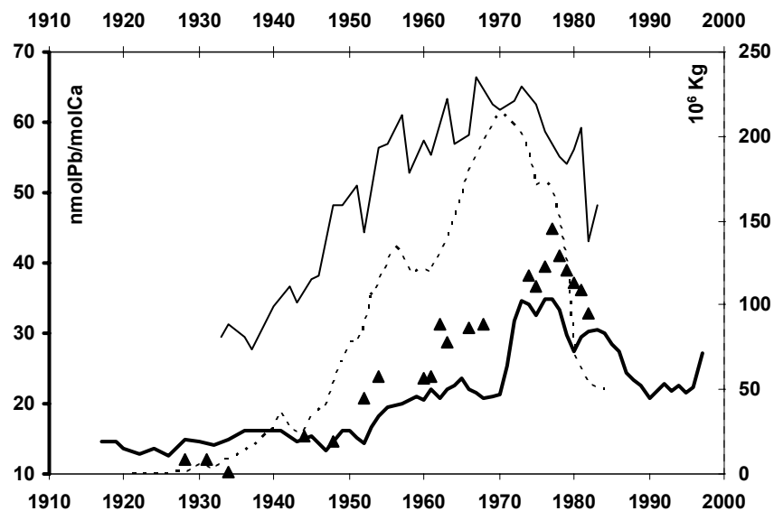
Figure 2. US Alkyl Lead Consumption (dashed line in 10^6\text{kg} ) and Lead Concentration data in Mona coral skeleton (solid line explained nmolPb/molCa) compared with Shen's results on Florida (▲) and Bermuda (medium line) corals.
