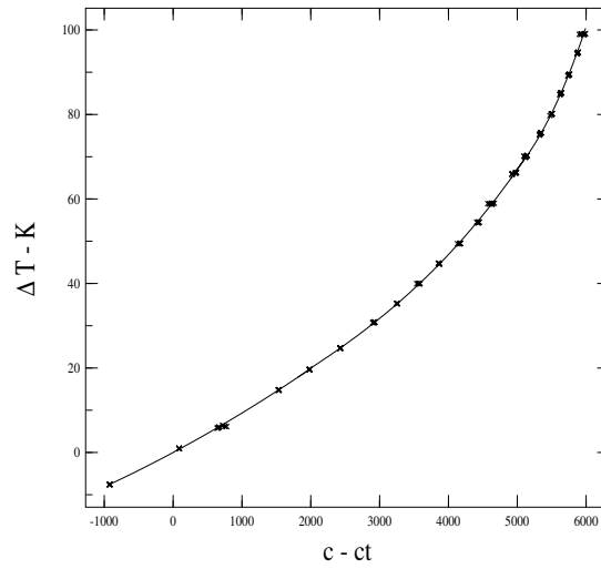
Figure 6: Temperature calibration for the broad-band channel at T_d = 19.6^\circ\text{C} performed on 04/04/1995. \Delta T = T_d - T_{cn} and c = C(T_{cn}) - C(T_d)
