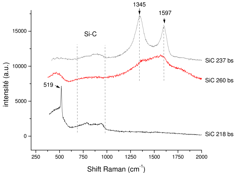
Figure IV-18 : Spectres Raman des nanopoudres brutes
