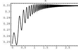
FIG. 5.9 – If we take into account a perfect fluid, k may reach a constant value during isotropisation.
