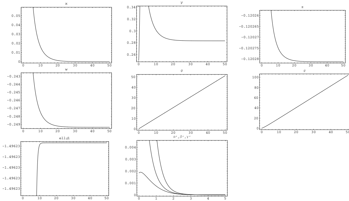
FIG. 5.6 — These figures, with -\Omega in abscissa, represent successively the behaviours of (x,y,z,w,\phi,\psi,\ell_{\psi_1}) for initial condition (x,y,z,w,\phi,\psi) = (-0.49,0.25, -0.12, -0.15,0.14,0.23) and parameters (U_0,k,m) = (3.2,1.25, -0.36) and a dust fluid. Note that \ell_{\phi_1} is a constant -k/\sqrt{3} = -0.721688 . The last figure shows the vanishing of \alpha, \beta and \gamma derivatives with respect to the proper time as it should be in case of metric functions convergence to a power law of time. If we take m = -2.36 , (11k^2 - 10km + 3m^2)/8 > 3 and class 1 isotropisation does not occur since x tends to a non vanishing constant
