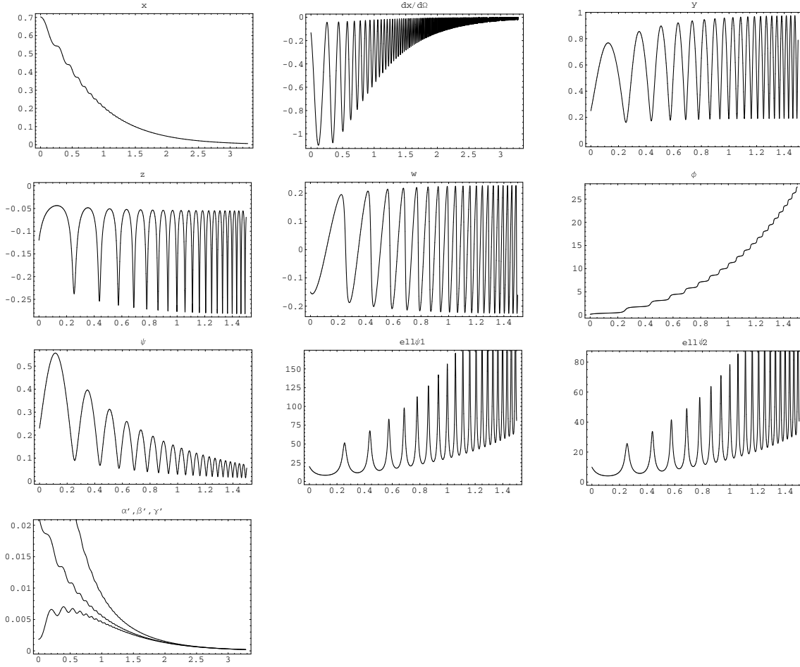
FIG. 5.8 — These figures, with -\Omega in abscissa, represent successively the behaviours of (x, \dot{x}, y, z, w, \phi, \psi, \ell_{\psi_2}, \ell_{\psi_2}) for initial condition (x, y, z, w, \phi, \psi) = (-0.70, 0.25, -0.12, -0.15, 0.14, 0.23) and parameters m = -2.3 . x is the only variable to reach equilibrium whereas y, z and w oscillates more and more as -\Omega increases. The scalar fields undergo damped oscillations whereas the oscillations for \ell_{\psi_2} and \ell_{\psi_2} increase. The last figure shows the vanishing of \alpha, \beta and \gamma derivatives with respect to the proper time as needed for isotropisation. Note that they oscillate.
