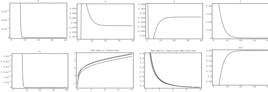
FIG. 6.9 – These figures represent the approach for class 1 isotropisation when \omega_0 = 2.3 , \omega_1 = 0.5 , n = -3.1 , m = 1.1 and p = 0.7 . k and \phi vanishes. \ell tends to 0.35 which is smaller than 3/2\gamma = 3/2
