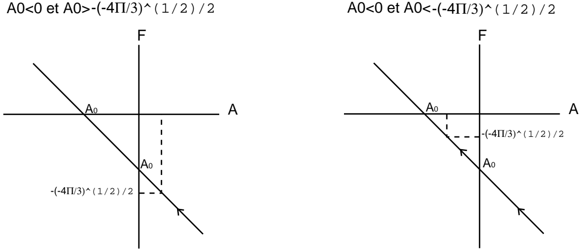
FIG. 5.3 – The string inspired theory when \omega < -3/2 , n < 0 and A_0 < 0 . F increases (this is indicated by the direction of the arrows on each straight line of the figures) from -\infty to -\sqrt{-4\Pi/3}/2 since (G^{-1})'' > 0 . On the first figure, this last value is smaller than A_0 . Then A is always positive and since G^{-1} > 0 , \alpha' is positive. The metric function e^\alpha is increasing. On the second figure, -\sqrt{-4\Pi/3}/2 is larger than A_0 . As long as F < A_0 , A > 0 and then when F > A_0 , A < 0 . Since A and \alpha' have the same sign we deduce that the metric function has a maximum.
