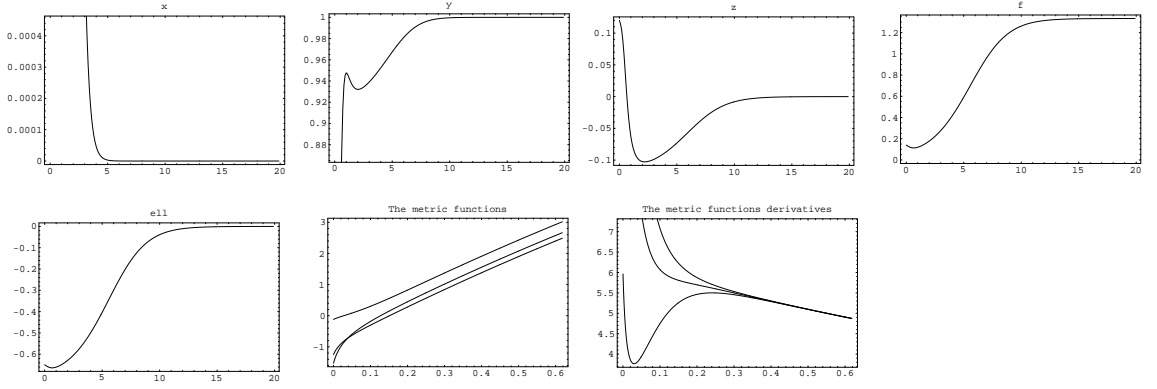
FIG. 6.2 – These figures represent the approach for class 1 isotropisation when \omega_0 = 2.3 , n = 1.5 and m = 1.1 . As expected, x tends to 0, \phi to the constant 2/n = 1.33 and \ell (here named ell ) to 0. The convergence of \phi to a constant is in accordance with the fact that U also tends to a constant and the Universe to a De Sitter model. In the Brans-Dicke frame, the derivatives of the metric functions \alpha , \beta and \gamma tend to the same behaviour showing isotropisation.
