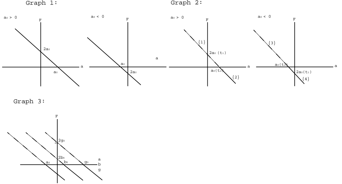
FIG. 4.1 – Figure 1 : solution of the first equation of (4.9) in the \alpha, \Phi plane depending on the sign of \alpha_0 . Figure 2 : the four different physically solutions of the first equation of (4.9). Figure 3 : representation of all the solutions of the equations (4.9) in the ((\alpha, \beta, \gamma), \Phi) plane.
