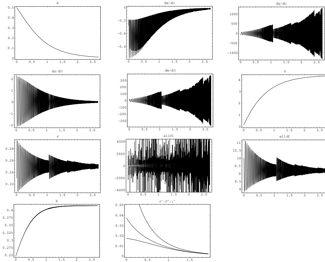
FIG. 5.10 — These figures, with -\Omega in abscissa, represent successively the behaviours of (x, \dot{x}, \dot{y}, \dot{z}, \dot{w}, \phi, \psi, \ell_{\psi_2}, \ell_{\psi_1}) for initial condition (x, y, z, w, \phi, \psi) = (0.49, 0.25, -0.12, -0.15, 0.14, 0.23) and parameters (\lambda, \eta) = (0.25, 0.25) . x, z and the scalar fields reach equilibrium whereas \ell_{\psi_1} undergoes non damped oscillations. The last figure shows the vanishing of \alpha, \beta and \gamma derivatives with respect to the proper time.
