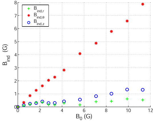
(a) \vec{B}_0 axial, \Omega = 8 Hz
