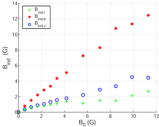
(c) \vec{B}_0 axial, \Omega = 17 Hz
