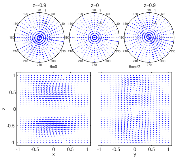
Fig. III.51: Projections de \vec{j}_2
