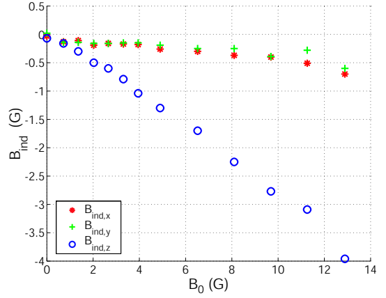
(b) \vec{B}_0 transverse, \Omega = 8 Hz
