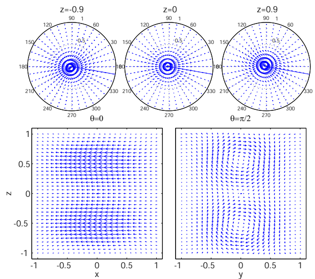
Fig. III.52: Projections de \vec{B}_2
