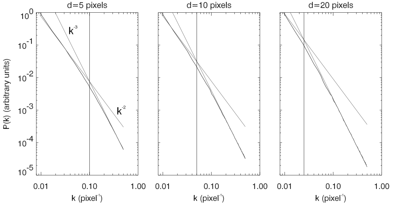
Fig. 8.—Power spectra of integrated emission slices of a \gamma_m = -3.0 density cube. The depths of the slices are d = 5, 10 , and 20 pixels, from left to right. The solid line is the power spectrum of the integrated density slice. The dotted lines indicate -3.0 and -2.0 slopes, and the vertical dashed line shows the 1/2d scale.
