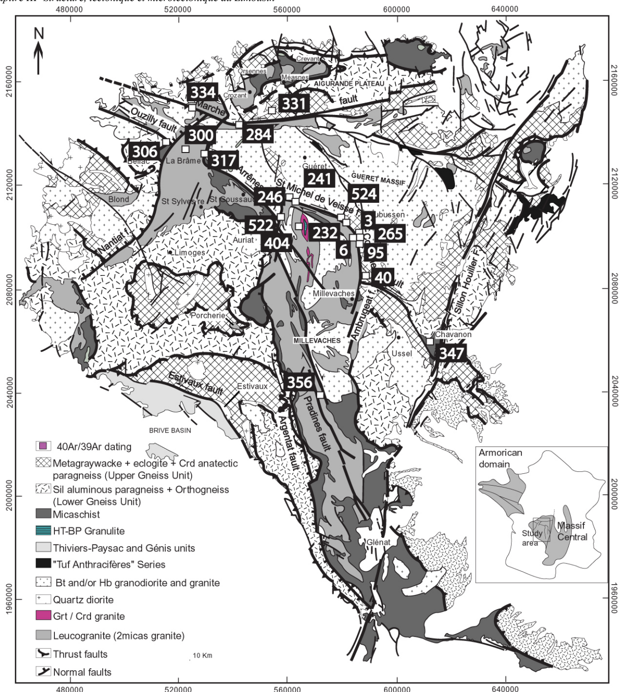
Figure 1 : Simplified geological map of the northwestern part of the French Massif Central with the location of 40 Ar/ 39 Ar dating.
