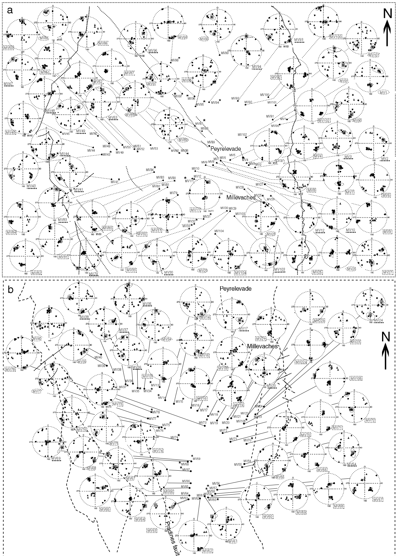
Figure 4 : Equal-area projection of AMS results for (a) the north part and (b) the south part of our study area in the Millevaches massif. The three main axes of the ellipsoid ( K_{max} \geq K_{int} \geq K_{min} ) are represented by squares, triangles and circles respectively with unweighted 95% confidence zones. The small symbols are for the specimen data, the large grey symbols are for the site average data.
