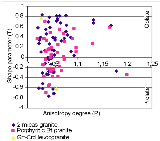
Figure 5: Plot of the shape (T) and anisotropy degree (P) parameters showing a well mixed pattern of the linear (prolate) and planar (oblate) shapes between the two principal types of granite.
