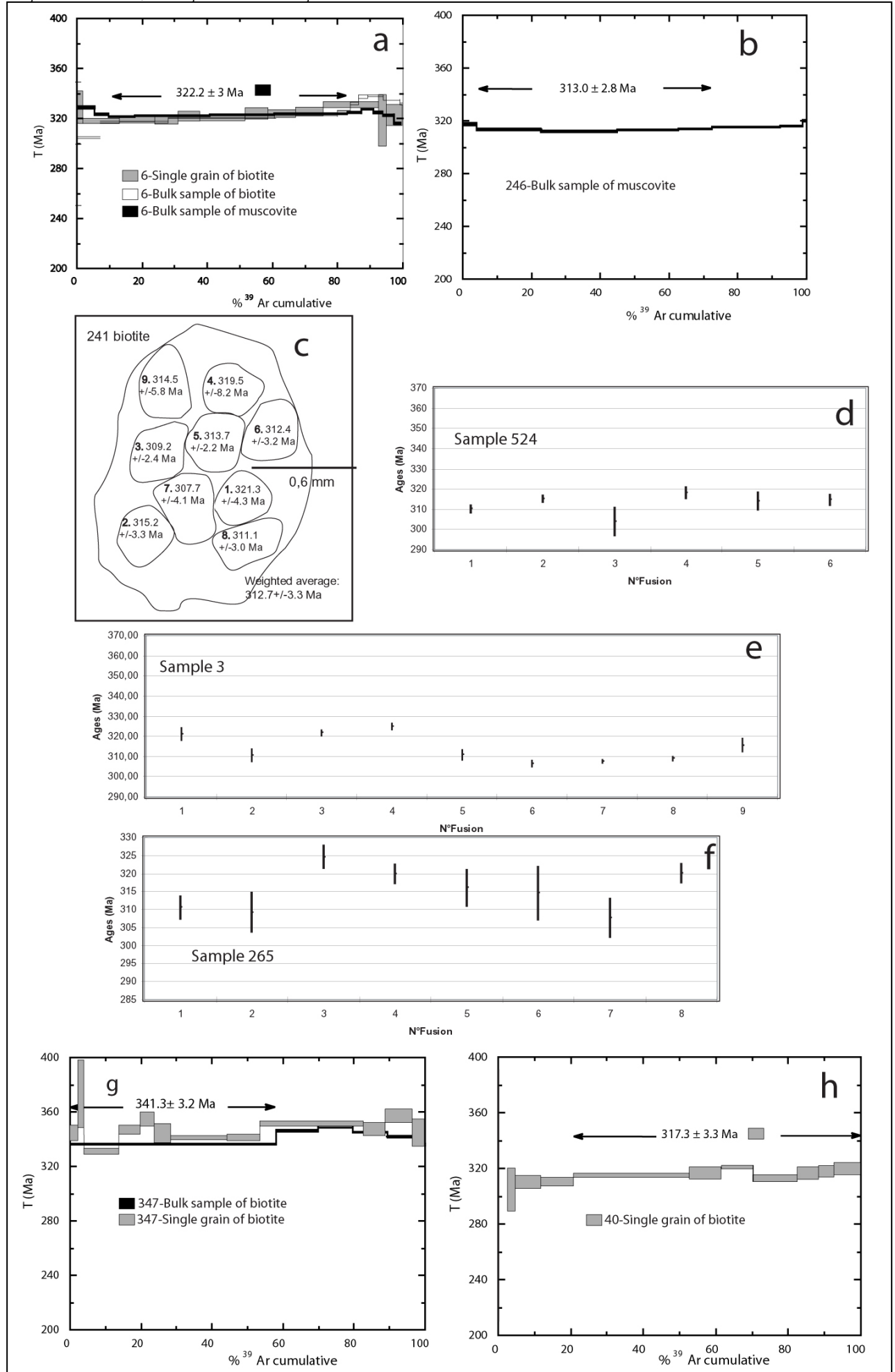
Figure 5: Felletin-La Courtine shear zone 40 Ar/ 39 Ar data. Sample location in Fig. 1
