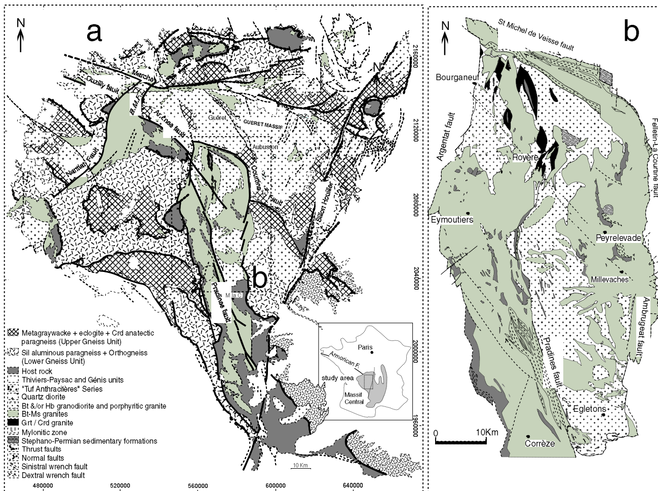
Figure1: Simplified geological map of the north-western part of the Massif Central, France.(a) Structural map of the study area in the French Massif Central. (b) Millevalches massif lithologic units map.
