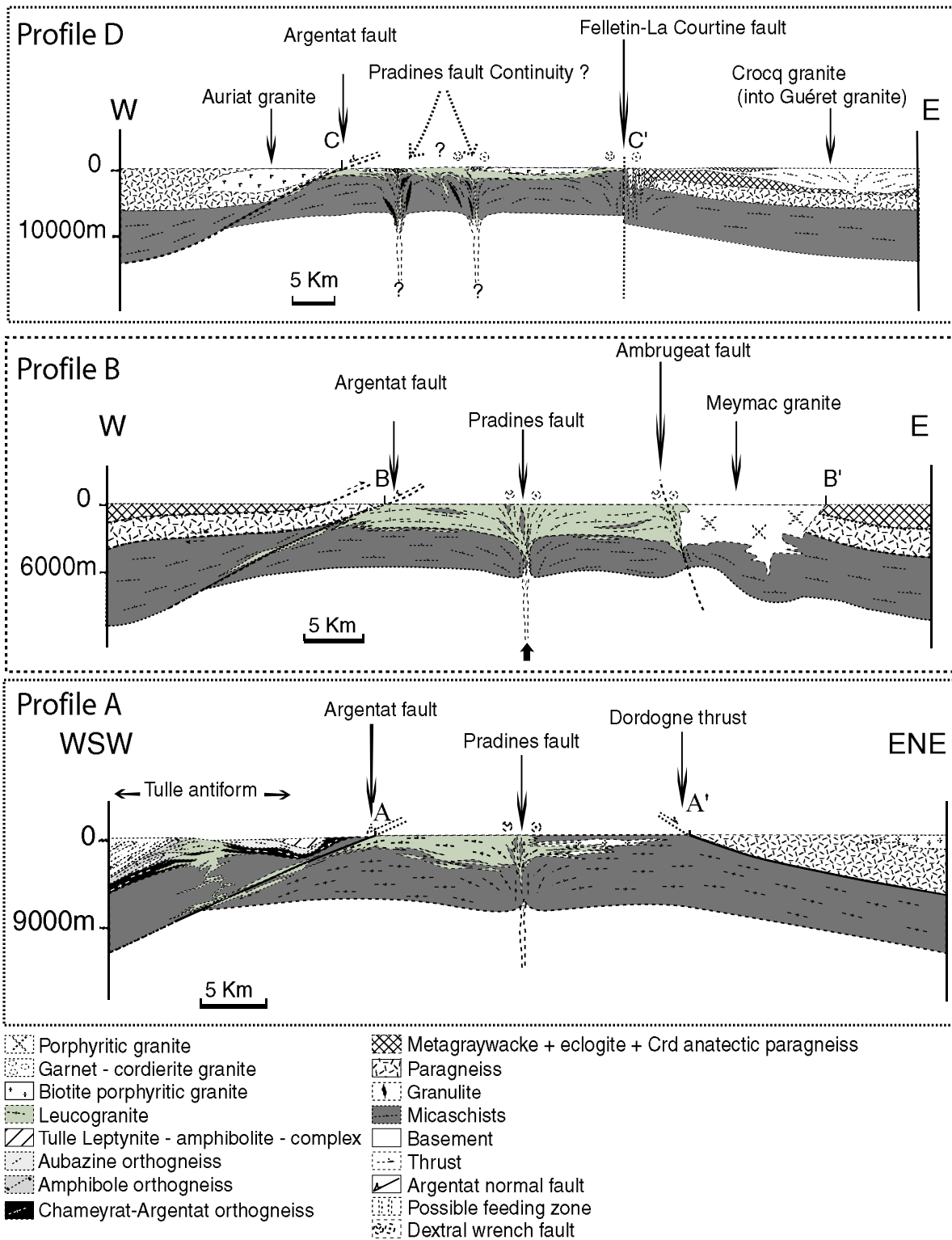
Figure 12: Sketch geological cross-sections, built from AMS and Gravity data, through the Millevaches granitic massif along profiles A, B and D (location on Figure 9).
