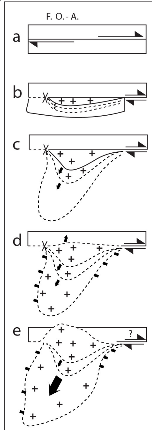
Figure 8: Model of Brême leucogranites emplacement (see description in the text)
