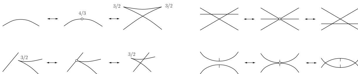
Figure 4.9: Generic singularities along isotopies of wave fronts.
