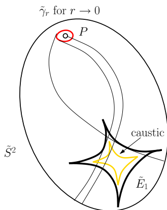
Figure 1.10: The Last Geometrical Theorem of Jacobi for envelopes.
