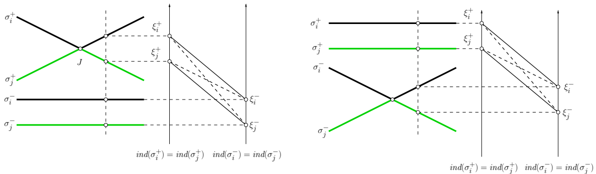
Figure 4.15: Morse diagram of forbidden configurations (II) and (III).
