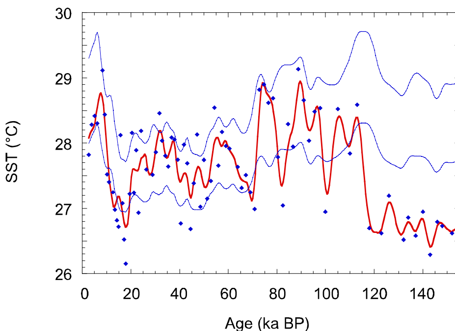
Figure 9 - Comparison of SST derived from foraminifera transfer function TROP-2 (filled diamonds) with alkenones SSTs derived using [Prah] et al., 1988] equation (thin line down) and the [Sonzogni et al., 1997] equation (thin line down) in the MD97-2138 core. The data were smoothed using a moving average of 2000 years after a resampling with a 500 years steps, to account for different sampling steps between these two proxies.
