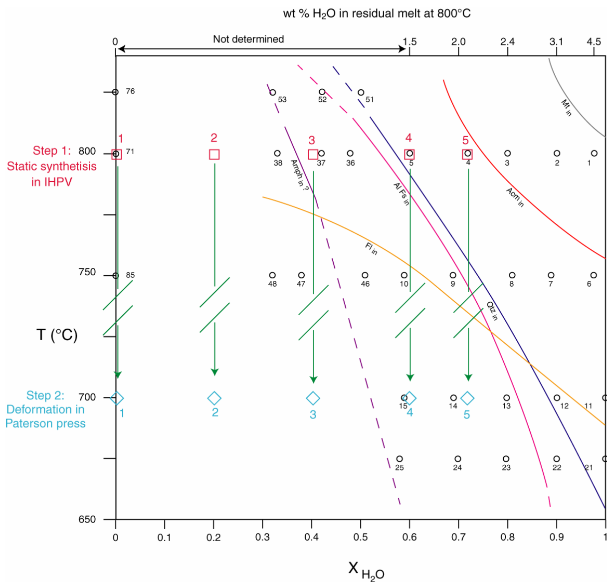
Fig 1: Phase relations of Eburru Rhyolite at 1.5 kbar
