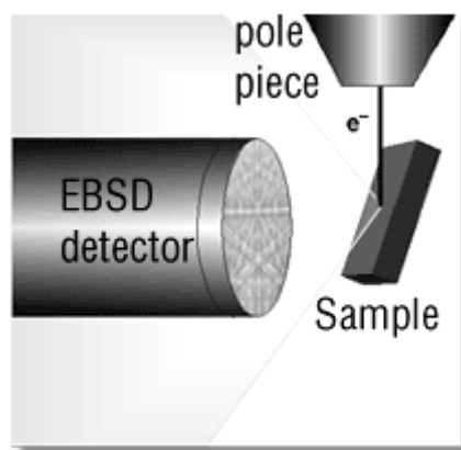
Figure II.18 – EBSD: position of the sample relative to the beam and the detector in the SEM chamber.
