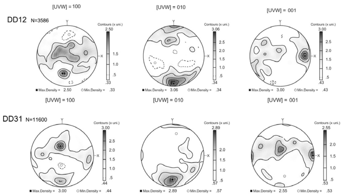
Figure III.13 – EBSD pole figure of forsterite samples: DD12, deformed to 24% at 2 GPa, 1300°C and 8 \times 10^{-5} s^{-1} and of DD31 deformed 25% at 6 GPa, 1300°C and 5 \times 10^{-5} s^{-1} . The compression axis is aligned with Y. Lower hemisphere equal-area projections, contours at intervals of 0.5 multiple of a uniform distribution.
