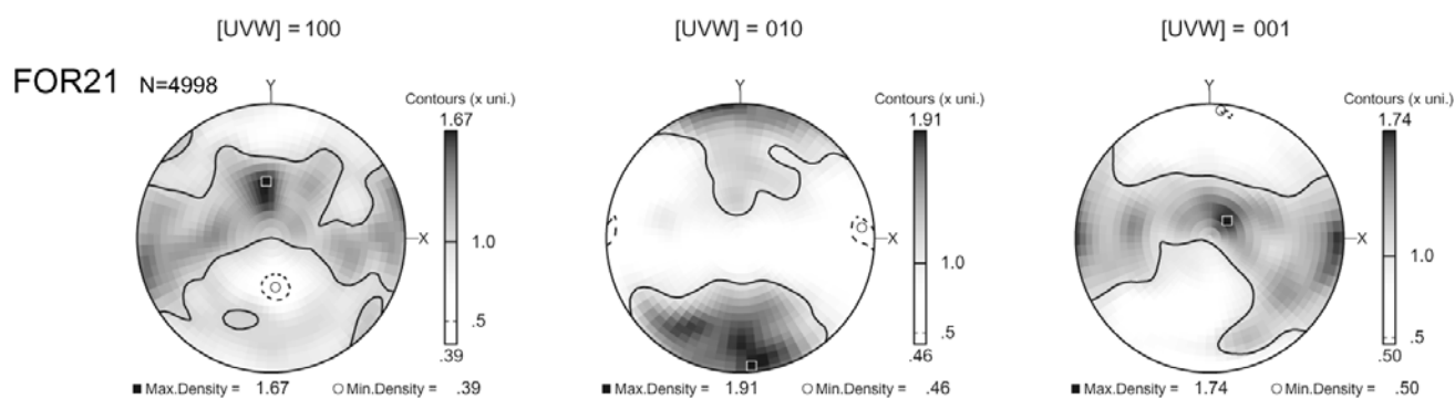
Figure III.21 – EBSD pole figure of crystal axis for forsterite sample (FOR21) deformed 10% at 4 GPa, 1300°C and 2.5 \times 10^{-5} s^{-1} . The compression axis is aligned with Y. Lower hemisphere equal-area projections, contours at intervals of 0.5 multiple of a uniform distribution.
