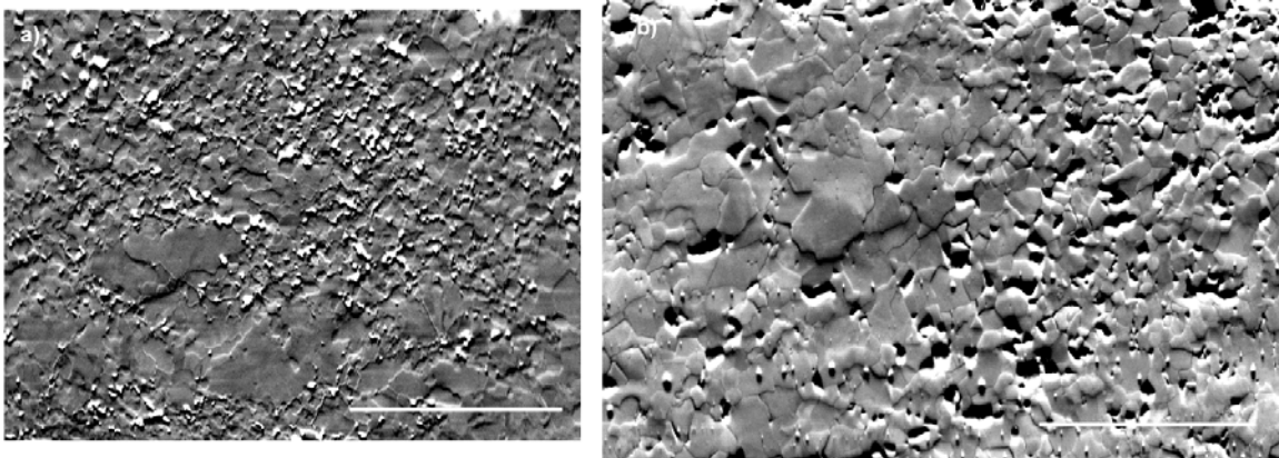
Figure III.32 – SEM pictures of ringwoodite samples (orientation contrast). Cross section, shear direction horizontal and shear sense dextral. The scale bar is equal to 20\text{ }\mu\text{m} a) After one minute at 22 GPa and 12300°C (Z367) – b) After three hours at 22GPa and 1300°C (Z341)
