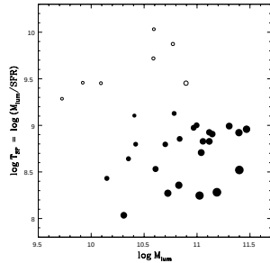
Fig. 11. Stellar mass versus time scale to duplicate the bulk of stars at a rate of the observed value. The stellar mass is derived from K band luminosity. The size of the point is scaled by the SFR. Nearby galaxies listed in Table 3 with available K band luminosity are shown with open circles for comparison.
