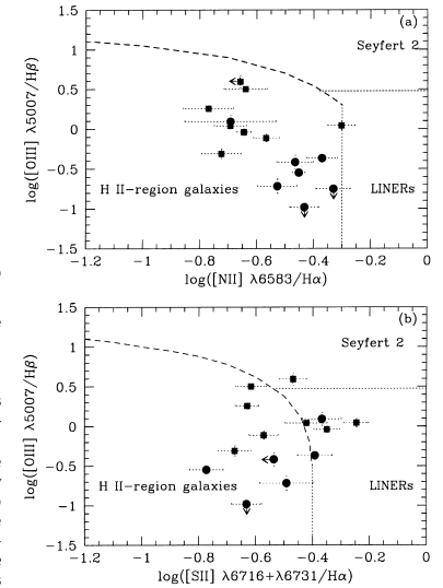
Fig. 7. a) [\text{O III}]/\text{H}\beta vs. [\text{N II}]/\text{H}\alpha diagnostic diagram for the sample galaxies; b) [\text{O III}]/\text{H}\beta vs. [\text{S II}]/\text{H}\alpha diagnostic diagram for the sample galaxies. Symbols as in Fig. 1.
