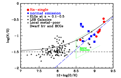
Fig. 10. N/O vs. O/H relations for the “CFRS Ha-single” galaxies (filled circles) and the “CFRS normal emission line” galaxies (filled squares), associated with the ELGs at z \sim 0.1-0.5 (open squares, from KZ99), the Low Surface Brightness (LSB) Galaxies (asterisks, from van Zee et al. 1997), the Local metal-poor Dwarf Irregular and Blue Compact Galaxies (BCGs) (open triangles, from Kobulnicky & Skillman 1996 and Izotov & Thuan 1999). All of them have been done using a spectral resolution comparable to ours. The dotted box for spiral galaxies is taken from KZ99. The horizontal dot-dashed line refers to the primary origin of nitrogen, the sloping dashed line refers to the secondary origin, and the solid line is the combined contribution of a (delayed) primary and a secondary component of nitrogen (taken from Vila-Costas & Edmunds 1993).
