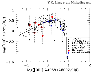
Fig. 8. The relations between [O II] \lambda 3727/H\beta in the “CFRS Ha-single” galaxies (filled circles) and the “CFRS normal emission line” galaxies (filled squares), together with a sample of the local H II regions and H II galaxies with different metallicities. The solid line shows the theoretical sequence from McCall et al. (1985), which fits the local H II galaxies well, with metallicity decreasing from the left to the right (also see Hammer et al. 1997).
