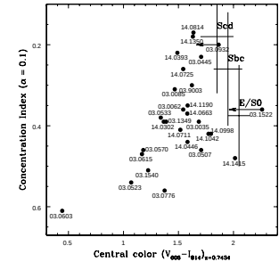
Fig. 13. Central color versus concentration index. The distributions (large crosses) of normal elliptical, Sbc and Scd galaxies are derived from a nearby galaxy sample (Frei et al. 1996). The modeling colors for the galaxies E, S0, Sbc and Irr at this redshift are 2.05, 1.88, 1.10 and 0.38 respectively (see Sect. 5.2.2). We assume that Sbc galaxies are bluer by 0.1 mag than E/S0 galaxies and Scd galaxies are 0.1 mag bluer than Sbc galaxies in the bulge color (de Jong 1996). A central color of 2.05 is adopted for E/S0 galaxies. The CFRS ID is labeled for each data point. A Spearman rank-order (S-R) correlation analysis reveals a correlation coefficient of -0.42 with a probability of 0.026 that the null hypothesis of no correlation is true.
