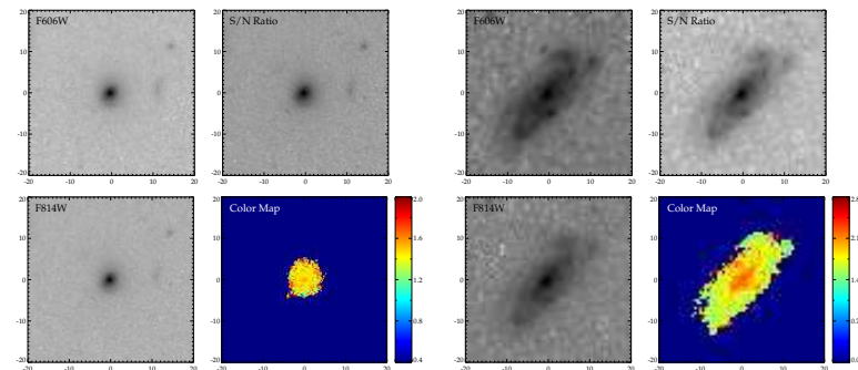
Fig. 5. V_{606} , I_{B14} , the color map S/N ratio, as well as color map images of elliptical galaxy 03.0037 at redshift 0.1730. (See the electronic edition for a color version of this figure.)
