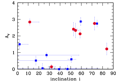
Fig. 6. The relations between extinction A_V and inclination i in the sample galaxies. Symbols as in Fig. 1.
