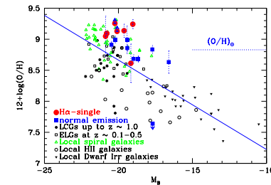
Fig. 9. Oxygen abundances vs. absolute blue magnitudes for the “CFRS Ha-single” galaxies (filled circles) and the “CFRS normal emission line” galaxies (filled squares), associated with the Luminous Compact Galaxies (LCGs) up to z \sim 1.0 (asterisks, from Gruel 2002 and Hammer et al. 2001), the Emission Line Galaxies (ELGs) at z \sim 0.1-0.5 (open squares, from Kobulnicky & Zaritsky 1999, KZ99), the Local Spiral Galaxies (open triangles, from ZKH), the Local H II Galaxies (open circles, from Telles & Terlevich 1997) and the Local Dwarf Irregular Galaxies (upside-down filled triangles, from Richer & McCall 1995). All of them have been done using a spectral resolution comparable to ours. The solid line is a linear least-squares fit to local irregular and spiral galaxies (from KZ99). Solar oxygen abundance is shown by the dotted line.
