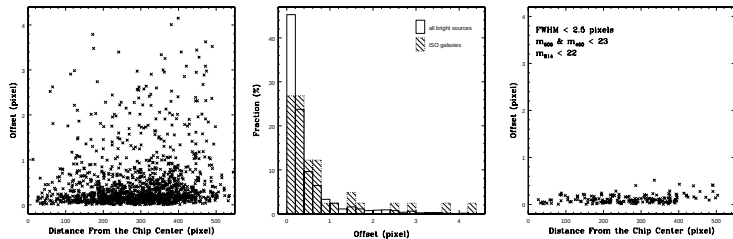
Fig. 4. Left panel: center offset of the bright sources ( m_{B14} \leq 22 ) between blue ( V_{606} or B_{450} ) and red ( I_{B14} ) image as a function of their positions in WFPC2 WF chip, expressed as the distance from the chip center. Middle panel: histograms of the center offset for all bright sources and for our ISOCAM-detected galaxies. Right panel: center offset for the point/point-like sources. In this panel, the mean value of the offset is 0.117 pixel with \sigma = 0.088 pixel.
