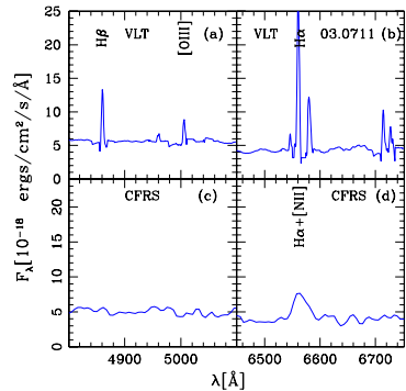
Fig. 3. a), b) Rest-frame spectra of CFRS03.0711 from the VLT observation around H \beta and [O III] wavelengths; c), d) the corresponding low-resolution CFRS spectra.
