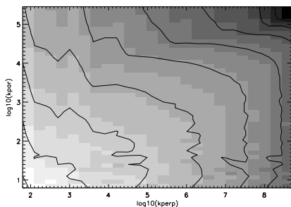
Figure 8. (k_{\perp}, k_{\parallel}) spectrum of the Z^+ field.
