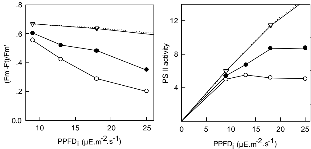
Figure 3. A : PS II quantum yield estimated from (F_m' - F_t) / F_m' as a function of light (incident photosynthetic photon flux density, PPFD i ) in stripped tobacco leaf discs. For anaerobic conditions leaves were flushed with N 2 in the dark during 2 min before light was turned on. Photosynthetic activity was measured 4 min after turning on the light. Anaerobic conditions: control (♦), ndhB - (●); Control and ndhB - under CO 2 -free air (▽;○). B : Photosynthetic flow estimated from (\Delta F / F_m' \times \text{PPFD}_i) as a function of light intensity. Anaerobic conditions: Control (♦); ndhB - (●); Control and ndhB - under CO 2 -free air (▽;○).
