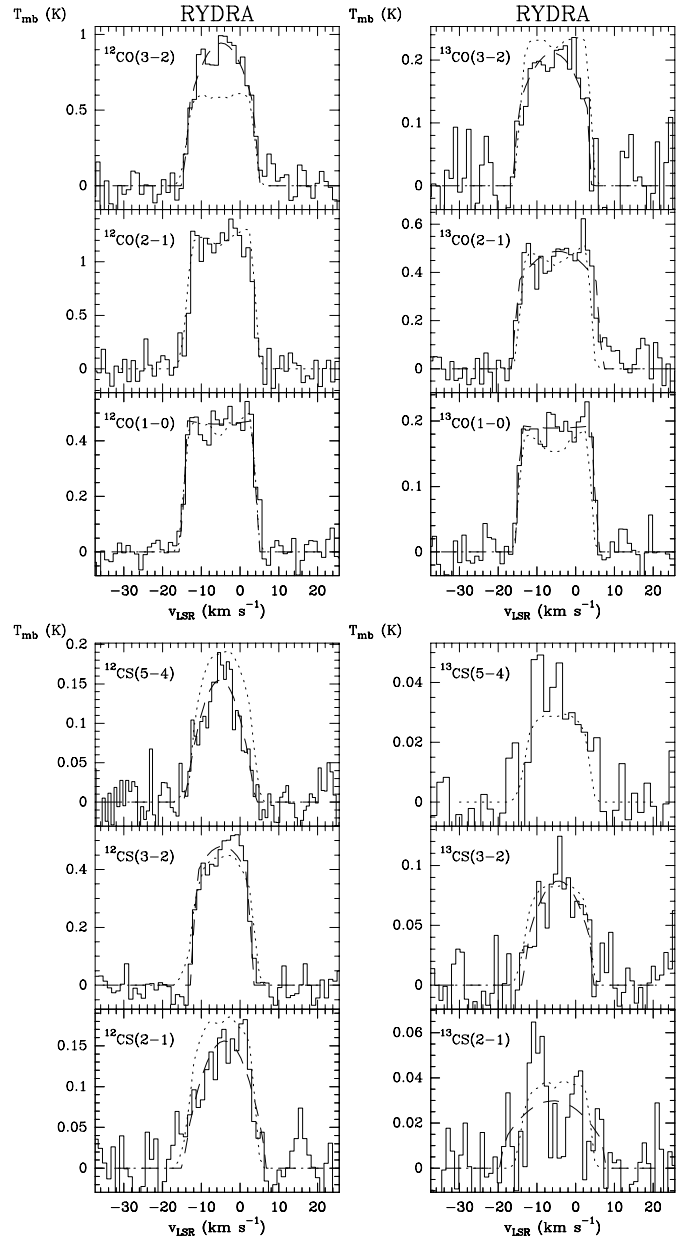
Fig. 2: Molecular spectra observed towards RY Dra. The source coordinates are \alpha(1950) = 12^{\text{h}} 54^{\text{m}} 28.1^{\text{s}} , \delta(1950) = 66^{\circ} 15' 52'' . The histograms represent observed spectra, the dashed lines model profiles and the dotted lines radiative transfer calculation results. On the observed spectra the velocity resolution has been smoothed to 1.1 \text{ km s}^{-1} .
