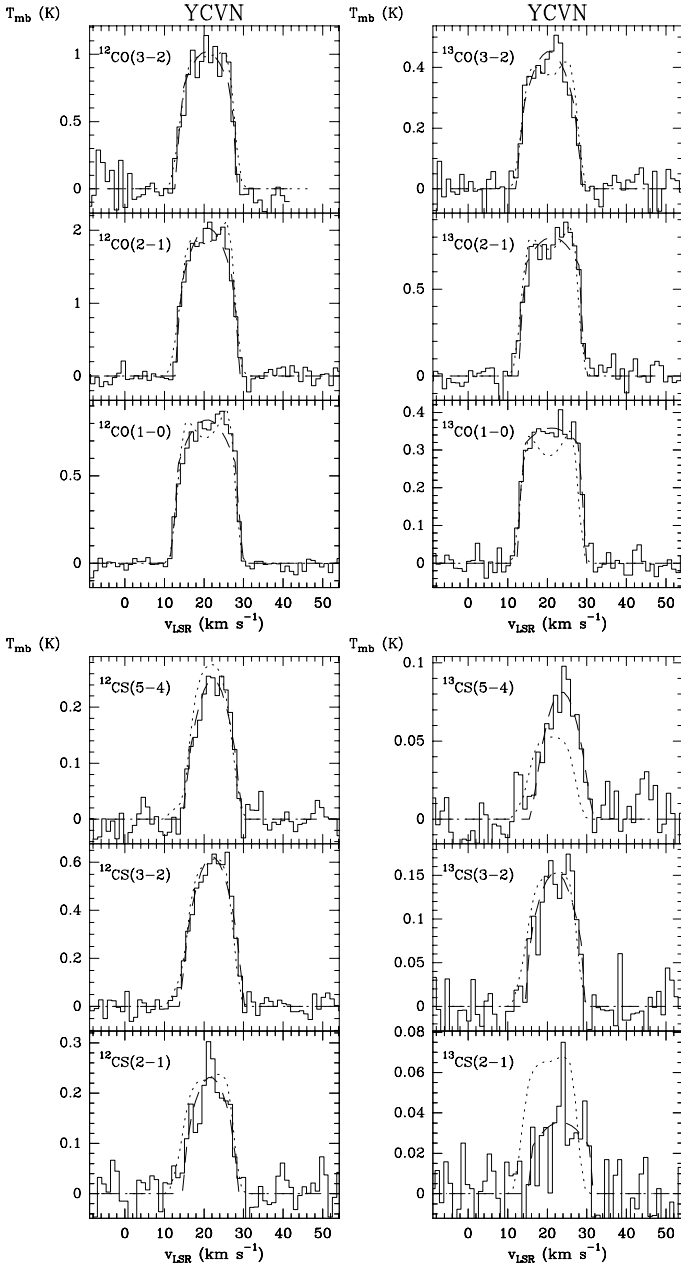
Fig. 1: Molecular spectra observed towards Y CVn. The source coordinates are \alpha(1950) = 12^{\text{h}} 42^{\text{m}} 47.0^{\text{s}} , \delta(1950) = 45^{\circ} 42' 48'' . The histograms represent observed spectra, the dashed lines model profiles and the dotted lines radiative transfer calculation results. On the observed spectra the velocity resolution has been smoothed to 1.1 \text{ km s}^{-1} .
