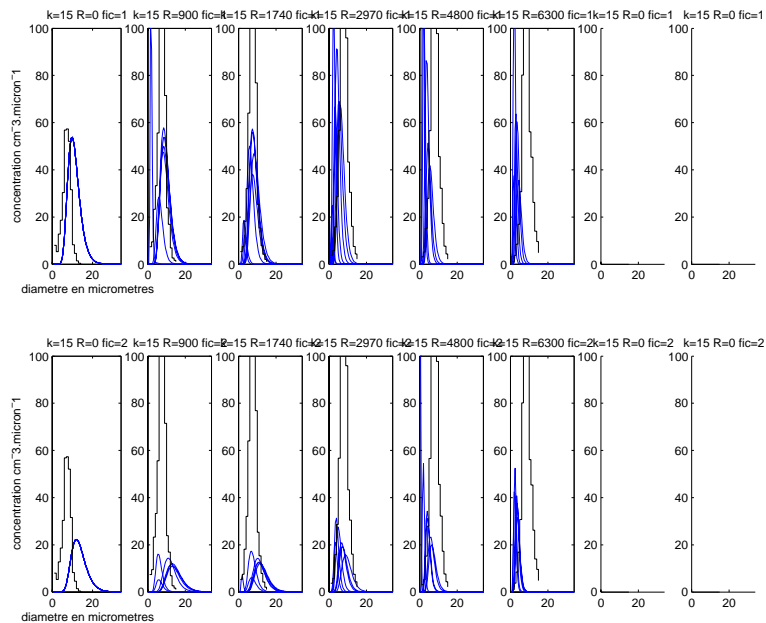
FIG. B.67 – Idem figure B.58. Palier n°5.
