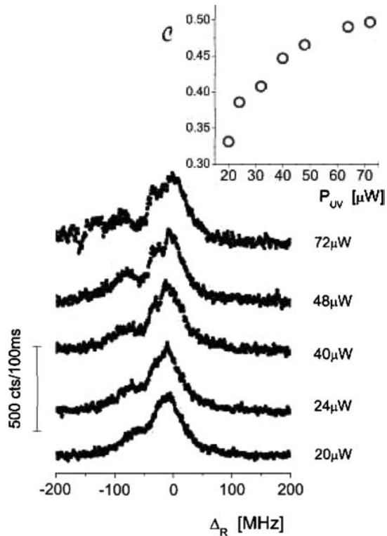
FIGURE 6 Fluorescence signal observed with counter-propagating laser beams. The graph shows the influence of the laser power on the level splitting; the offset of the curves is due to the varying laser power. The applied blue laser powers are marked on the right-hand side of the curves, where the lowest value corresponds to about 2\Gamma_B while the highest power is equivalent to 4\Gamma_B . The inset shows the increasing contrast of the fluorescence signal with higher laser power
