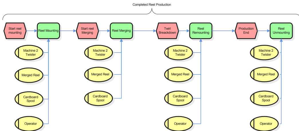
Figure 9.6 - EPC model of the Completed Reel Production
