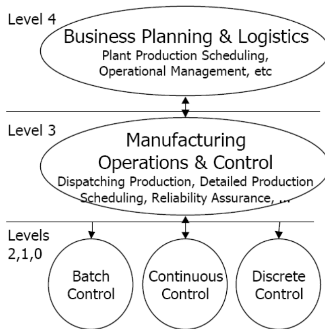
Figure 6.4 - Functional Hierarchy
