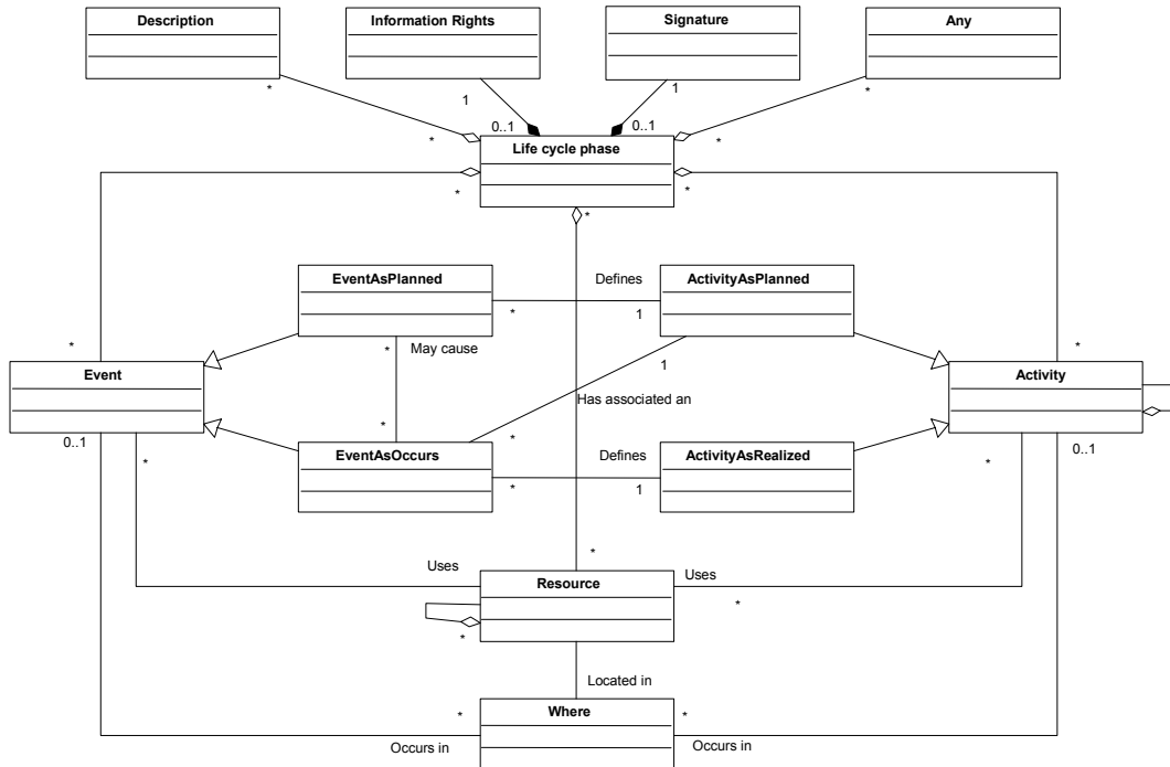
Figure 8.13 - Product Life Phase model
