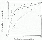
Fig. 3. Cu(111) surface composition versus Cu bulk composition for Cu-Ni alloys: comparison between the experimental and theoretical results. Regular model: T = 973 K, (—) surface; (— — —) 2nd plane. Monte Carlo calculations: T = 973 K, (+) surface; (+) 2nd plane. Experimental results: (□) AES, T = 873 K, ref. [18]; (+) AES, T = 873 , 2nd plane, ref. [18]; (▲) ISS, T = 773 K, ref. [19]; (◇) ISS, T = 673 K, ref. [19]; (○) AP FIM, T = 823 K, refs. [20,21]; (●) AP FIM, T = 923 K, refs. [20,21]; (⊕) AP, T = 870-920 K, ref. [22].
