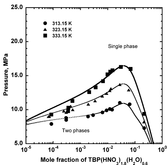
Figure 8. Phase diagram of \text{TBP}(\text{HNO}_3)_{1.8}(\text{H}_2\text{O})_{0.6} in \text{SF-CO}_2 .
