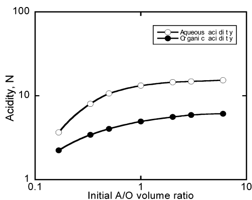
Figure 1. Acidities of the aqueous and organic phases. The x axis is the initial volume ratios of 15.5 M \text{HNO}_3 to 98% TBP. (○) Aqueous acidity is defined as moles of \text{H}^+ per liter of aqueous solution. (●) Organic acidity is defined as moles of \text{H}^+ per liter of organic solution.
