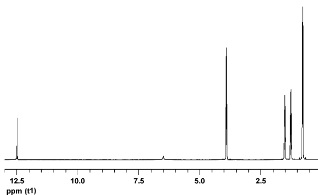
Figure 6. PNMR spectrum of \text{TBP}(\text{HNO}_3)_x(\text{H}_2\text{O})_y in \text{CDCl}_3 . The complex was prepared by mixing 4 mL of TBP and 1 mL of 15.5 M \text{HNO}_3 ; volume ratio of \text{TBP}(\text{HNO}_3)_x(\text{H}_2\text{O})_y to \text{CDCl}_3 = 1:1 .
