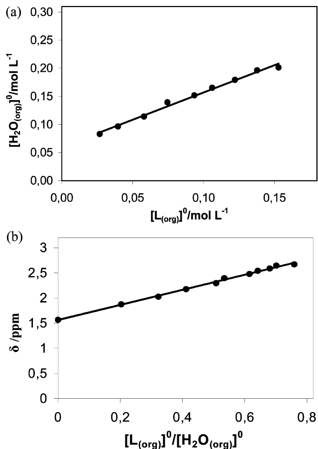
Figure 2. Linear relationship between (a) the total water and 18-crown-6 concentrations in chloroform ( [\text{H}_2\text{O}_{(\text{org})}]^\circ = 0.9704 - [\text{L}_{(\text{org})}]^\circ + 0.0601 ; correlation coefficient r = 0.9955 ) and between (b) the observed chemical shift of water and the ratio [\text{L}_{(\text{org})}]^\circ/[\text{H}_2\text{O}_{(\text{org})}]^\circ in chloroform (eq 7) ( \delta = 1.5015[\text{L}_{(\text{org})}]^\circ/[\text{H}_2\text{O}_{(\text{org})}]^\circ + 1.5611 ; r = 0.9982 ).
