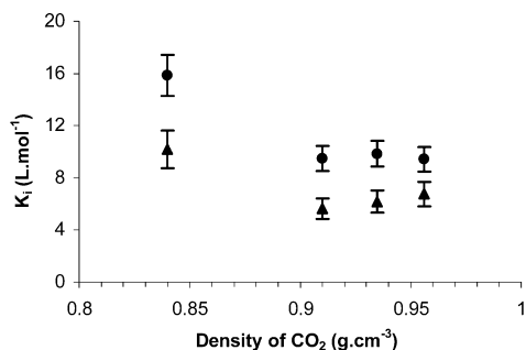
Figure 5. Density effect on equilibrium constants K_s (●) and K_b (▲). The pressure varies from 200 to 400 bar at constant temperature (40 °C). [18C6] = 41 mmol·L -1 . [D 2 O] = 49 mmol L -1 .
