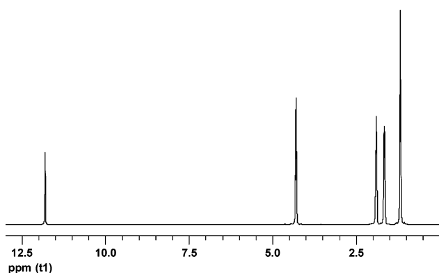
Figure 4. Typical PNMR spectrum of \text{TBP}(\text{HNO}_3)_x(\text{H}_2\text{O})_y with a \text{D}_2\text{O} insert. The sample was prepared by mixing 1.0 mL of 15.5 M \text{HNO}_3 with 4.0 mL of 98% TBP.
