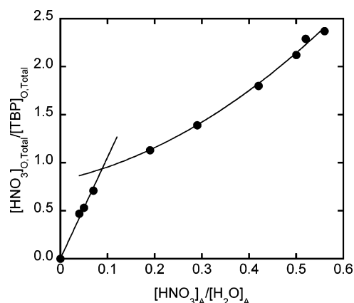
Figure 2. Plot of the [\text{HNO}_3]/[\text{TBP}] ratio in the TBP phase against the [\text{HNO}_3]/[\text{H}_2\text{O}]_A ratio in the equilibrated aqueous phase.
