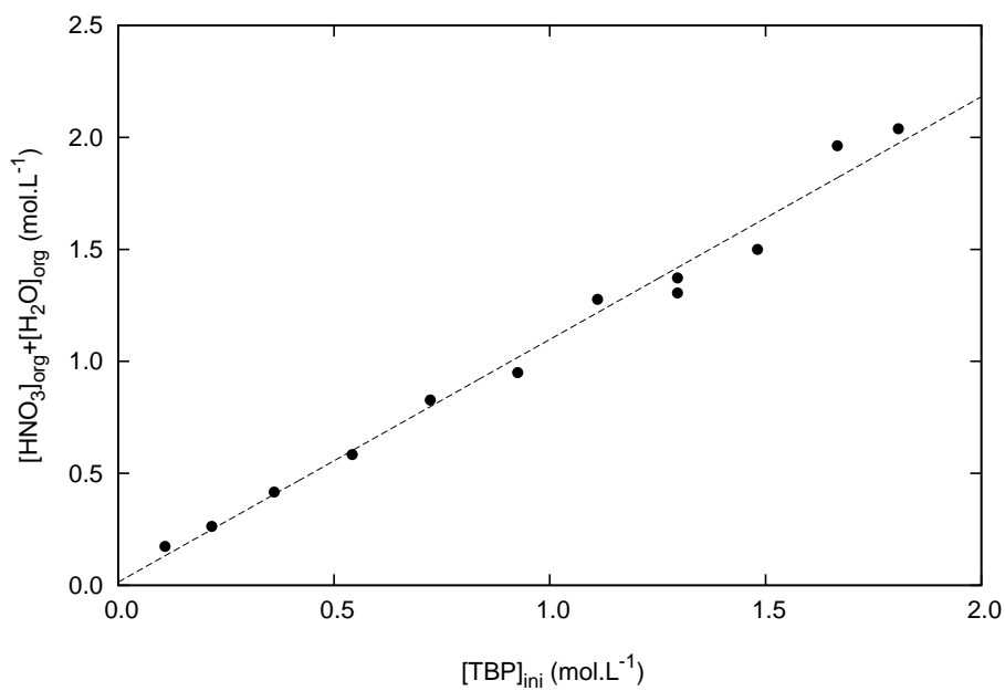
Figure 2.30: Total water and nitric acid concentration in \text{CDCl}_3 versus initial TBP concentration.
