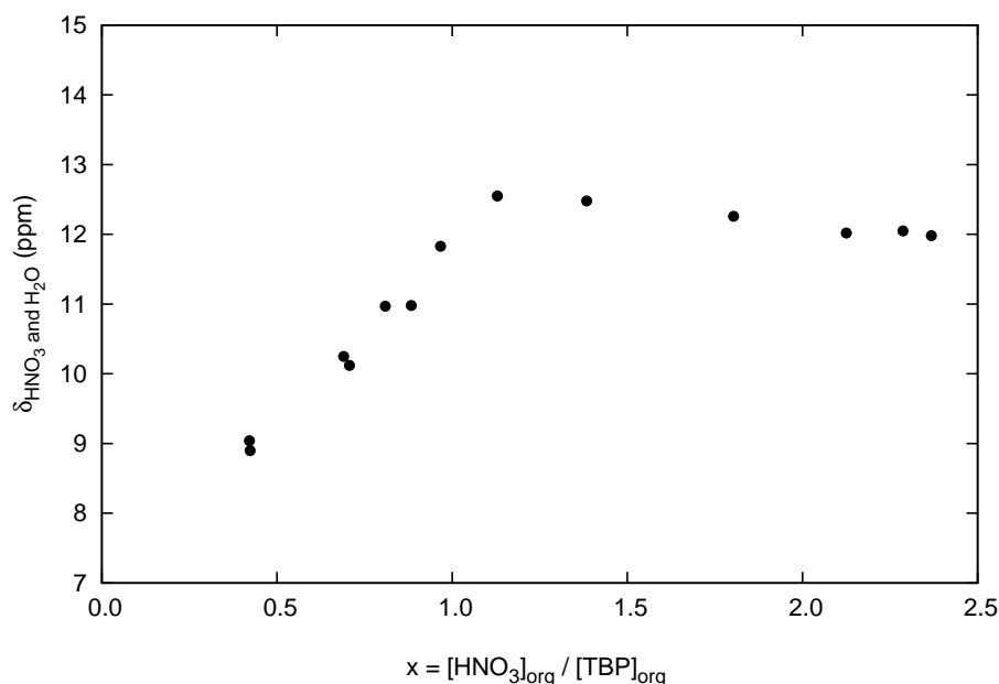
Figure 2.23: Chemical shift observed of nitric acid and water in TBP versus the mole ratio of nitric acid on TBP in the organic phase.
