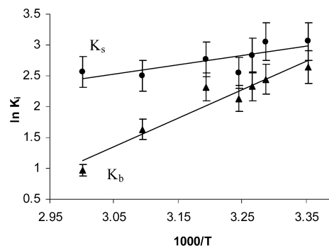
Figure 6. Dependence of \ln K_s (●) and \ln K_b (▲) on 1000/T at 200 bar for [18C6] = 41 mmol L -1 and [D 2 O] = 49 mmol L -1 .
