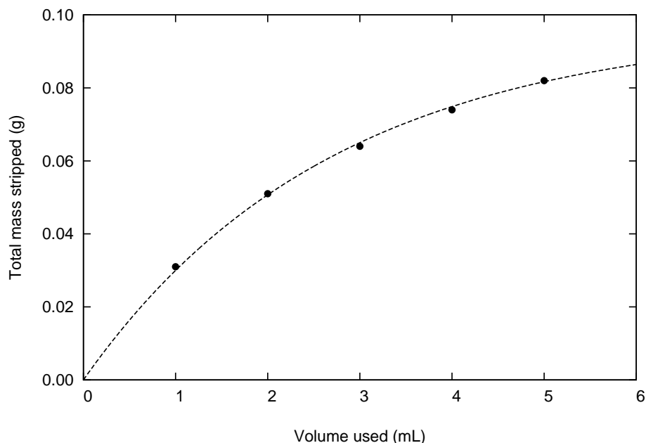
Figure 2.36: Total mass of uranium stripped versus total volume of water used. The line is a guide for the eyes and does not have any theoretical or analytical value.
