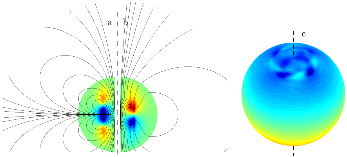
FIG. 5.6 – Growing magnetic field in kinematic dynamos for E = 10^{-8} . (a) and (b) are meridional cut of the sphere showing the axisymmetric part of the magnetic field. The solid lines are the poloidal field lines and the color map represent the azimuthal field. (a) shows a quadrupole field obtained at Ro = 0.02 and P_m = 0.005 . (b) shows a dipole field obtained at Ro = -0.02 and P_m = 0.003 . (c) is a spherical map of the radial magnetic field at the surface of the core, corresponding to case (b), the dashed line being the rotation axis. The corresponding vorticity fields are given in figure 5.3cd.
