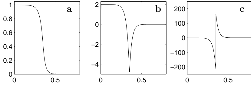
FIG. 3.15 – Basic state axisymmetric flow profiles (solution of eq. 3.17), as a function of radius r for E = 10^{-6} and a split-sphere geometry with r_0 = 0.35 . (a) rotation velocity U/r ; (b) vorticity \Omega ; (c) radial derivative of vorticity \frac{\partial\Omega}{\partial r} .
