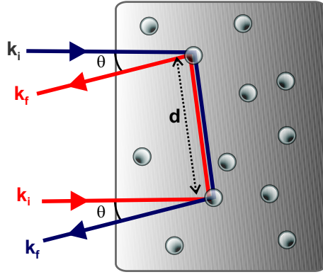
Figure 2.20: Double scattering event.
