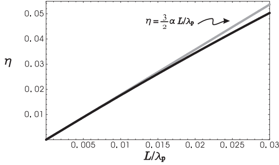
Figure 2.5 : A plot of the corrective coefficient \eta as function of L/\lambda_p . The graphics shows that in the short distances limit ( L \ll \lambda_p ) when the metal is described by the plasma model the corrective factor linearly depends on the rapport L/\lambda_p (see the gray curve). The change in the power law of the Casimir energy generated in the limit L \ll \lambda_p by corrective factor recalls Casimir-Polder-Van der Waals interactions behavior.
