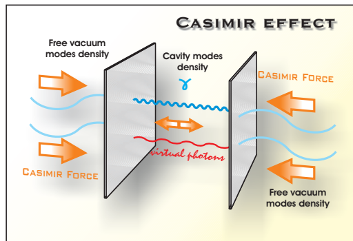
Figure 9 : An artist view of the Casimir effect. Two flat plan parallel mirrors, which are facing each other in quantum vacuum, are attracted to each other. As we will see later, the Casimir effect is the result of the competition between the intracavity and external vacuum radiation pressure. The intracavity spectral density is modified by the presence of the mirrors with respect to the external one.
