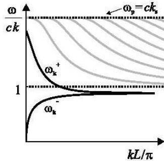
FIG. 2. Mode plot of the two plasmonic modes \omega_k^- and \omega_k^+ (black lines) in the sector \omega < ck and of photonic modes (gray lines) in the sector \omega > ck for ck = 0.5\omega_p . Modes are presented through their frequency as a function of kL/\pi .
