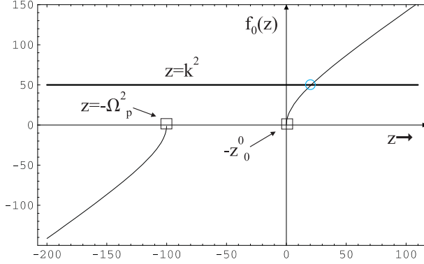
Figure 4.4 : A plot of f_0(z) . We can see that the solution of Eq.(4.4.11) besides in the evanescent region and it is unique.
