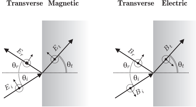
Figure 1.4 : A schematic representation of the reflection-transmission process for a plane wave incoming on an interface between two dielectric media. The TE and the TM modes have been represented separately. For the TE mode the electric vector is orthogonal to the incidence plane while for the TM mode it lays inside the incidence plane.
