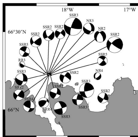
Fig. 7. Selection of focal mechanisms of earthquakes for the nine different determined regimes (SSR: strike-slip regime, NR: normal regime, RR: reverse regime). For all the regimes, excepted NR4 and RR3 regimes, only focal mechanisms of earthquakes with a magnitude bigger than M_L 2.5 are shown. For NR4 and RR3 regimes, only two focal mechanisms of earthquake are shown with respectively a magnitude of M_L 2.1 and M_L 1.6, respectively. The size of the balls is proportional to the magnitude of the earthquake.
