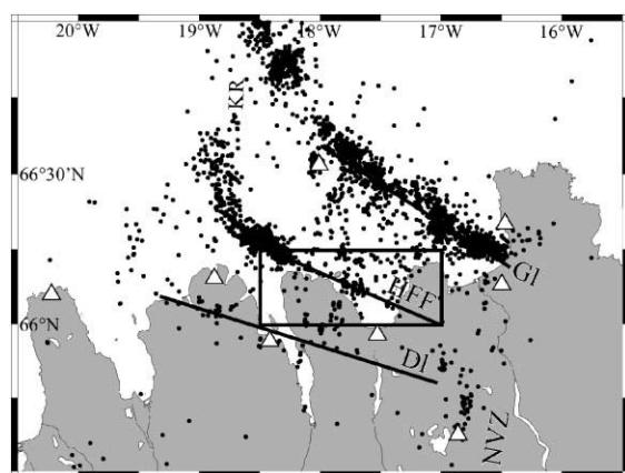
Fig. 2. Seismic map of the Tjörnes Fracture Zone for the period 1995–1997. The Dalvík lineament (DI), the Húsavík–Flatey Fault (HFF) and the Grímsey lineament (GI) are underlined by black lines. Earthquakes of magnitude superior or equal to 1 are represented as black dots. The rectangle includes earthquakes used in this paper. White triangle: seismometers of the SIL network.
