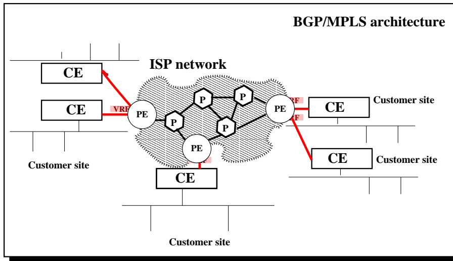
Figure 2.16. BGP/MPLS architecture
