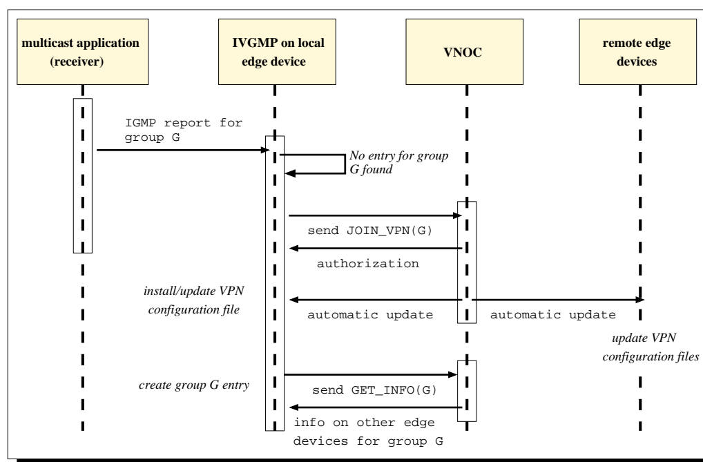
Figure 4.2. Joining a Multicast Group as a Client.
