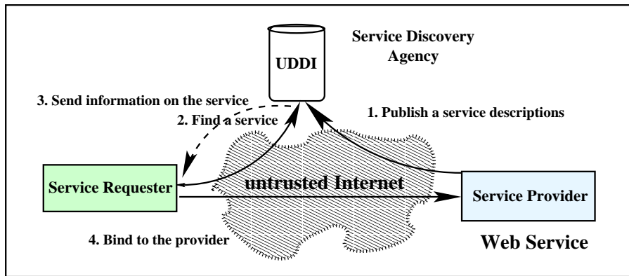
Figure 6.1. Web Service Architecture.
