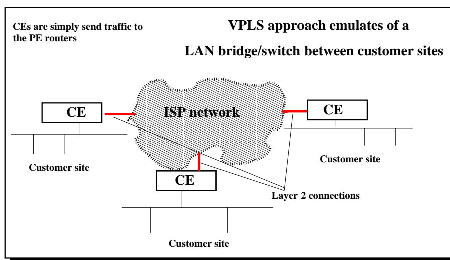
Figure 2.13. VPLS approach
