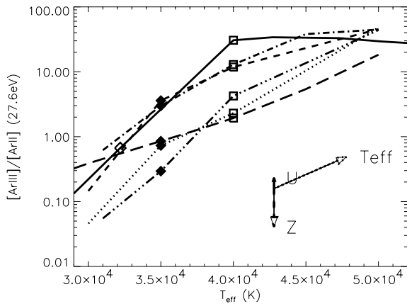
Fig. 11. Variation of the excitation diagnostic [\text{Ar III}/\text{II}] according to the T_{\text{eff}} of the ionizing star. Codes are the same as in Figs. 2, 3. The set of arrows have the same meaning as in Fig. 6, for WM-Basic models only.
