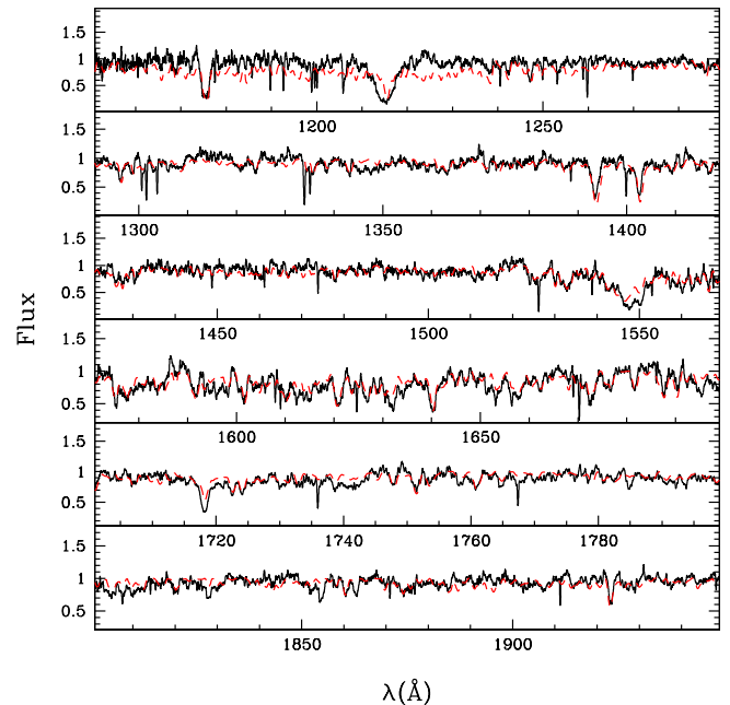
Fig. 3. Best fit (red dashed line) of the UV spectrum (black solid line) of HD 38666. For this model, \dot{M} = 10^{-9.5} M ⊙ yr -1 , v_{\infty} = 1200 km s -1 and \log L_X/L_{\text{bol}} = -6.87
