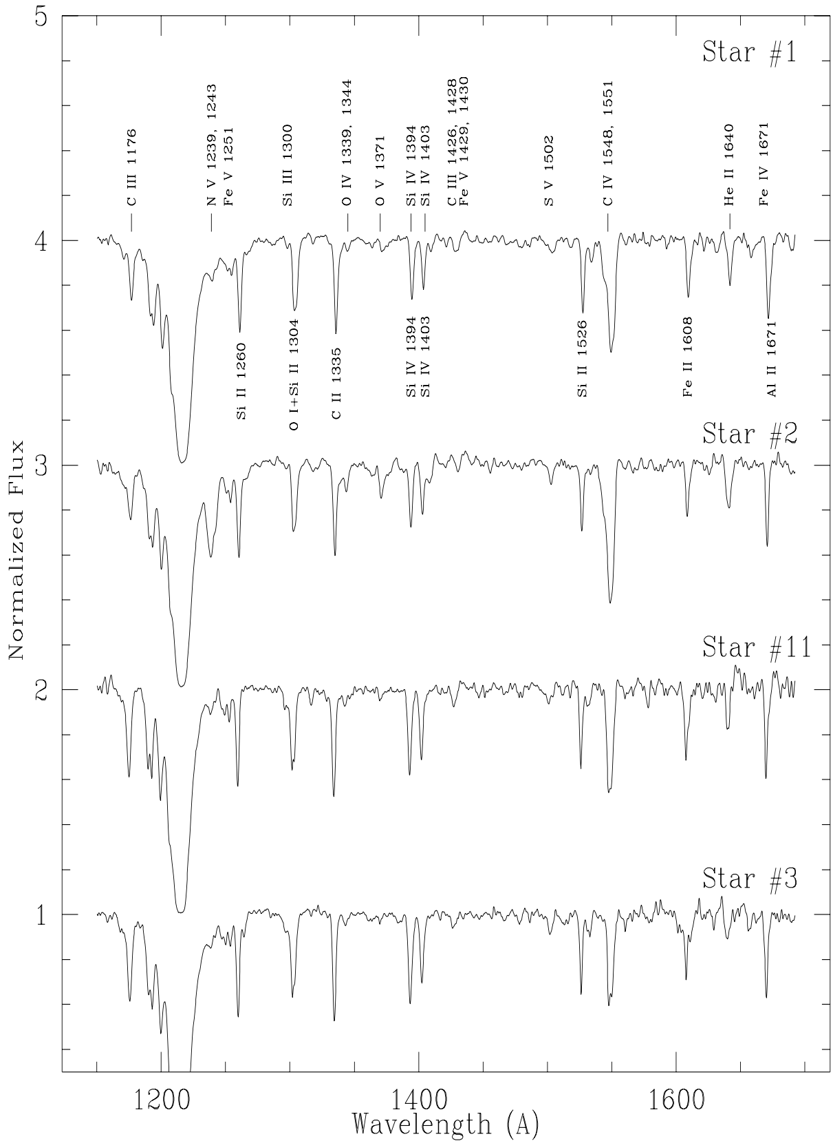
Fig. 1. Rectified HST /STIS ultraviolet spectrograms of the four brightest stars in SMC N81. The prominent absorption feature at \lambda 1210 \text{\AA} is due to the Ly \alpha . The wind profiles are indicated with tick marks and the features possibly contaminated by an interstellar component are labelled below the lines.
