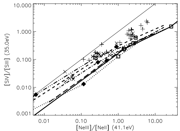
Fig. 5. Same as Fig. 3 for the excitation sensitive line ratio [\text{S IV/III}] versus [\text{Ne III/II}] .
