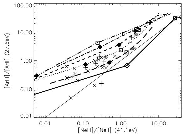
Fig. 4. Same as Fig. 3 for the excitation sensitive line ratio [\text{Ar III/II}] versus [\text{Ne III/II}] .
