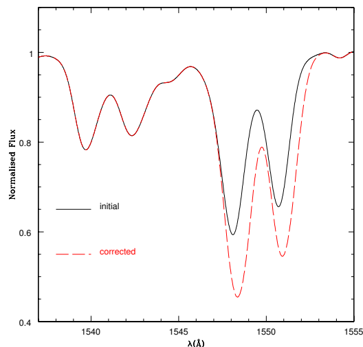
Fig. 1. Interstellar C IV component addition: the black solid line shows the C IV \lambda\lambda 1548,1551 profile of a CMFGEN model, and the red long dashed line is the resulting profile after including the IS absorption. A convolution has been performed to take into account the instrumental resolution ( 1.2 \text{ \AA} ). The parameters used to model the interstellar component are: \log(N(\text{C IV})_{\text{gal}}) = 14.4 , \log(N(\text{C IV})_{\text{SMC}}) = 14.5 and v_{\text{SMC}} = 140 \text{ km s}^{-1} .
