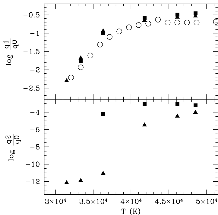
Figure 4.7: Ratio of He I ionising flux ( q_1 , upper panel) and He II ionising flux ( q_2 , lower panel) to Hydrogen ionising flux ( q_0 ) of CMFGEN models (filled triangles), CoStar models (filled squares) and from Vacca, Garmany & Schull (1996) (open circles).
