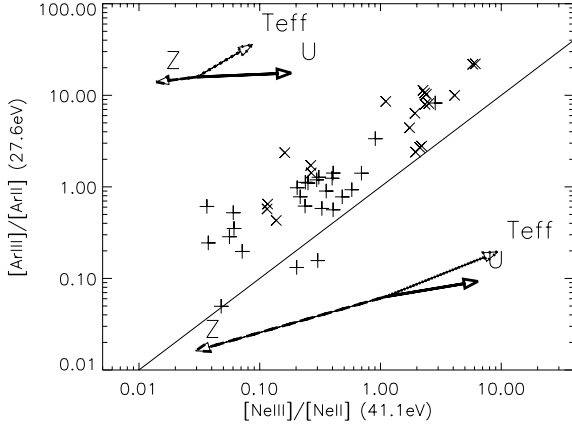
Fig. 6. Increase of the excitation diagnostics [\text{Ar III/II}] versus [\text{Ne III/II}] , when \log(\bar{U}) is increased from -2.6 to -0.8 (solid arrows), when the metallicity of the gas is increased from half solar to twice solar (dashed arrows), and when T_{\text{eff}} is increasing from 35 to 40 kK (dotted arrows). Upper set of arrows are for BlackBody models, and lower set for WM-Basic models. In the latter case the metallicity is changes coherently for both the gas and the star. Codes are the same than in Figs. 2, 3.
