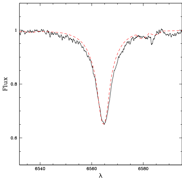
Fig. 2. Best fit (red dashed line) of the observed H \alpha line (black solid line) of HD 38666. We have derived \dot{M} = 10^{-9.5} M ⊙ yr -1 and v_{\infty} was 1200 km s -1 .
