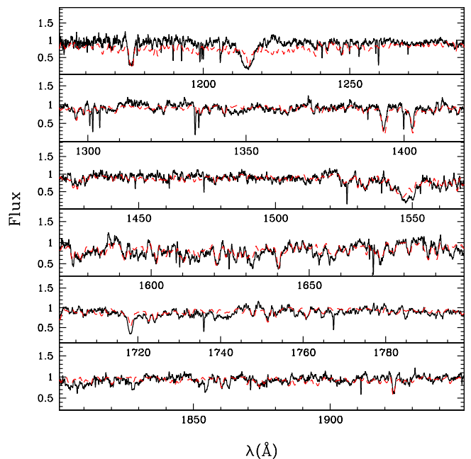
Fig. 3. Best fit (red dashed line) of the UV spectrum (black solid line) of HD 38666. For this model, \dot{M} = 10^{-9.5} M ⊙ yr -1 , v_{\infty} = 1200 km s -1 and \log L_X/L_{\text{bol}} = -6.87
