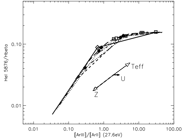
Fig. 7. Correlation between \text{He I } 5876 \text{ \AA}/\text{H}\beta and [\text{Ar III/II}] . The line styles are the same as in Fig. 2. Arrows have the same meaning as in Fig. 6, for WM-Basic models only.
