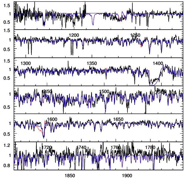
Fig. 23. Same as Fig. 22 for the UV range.
