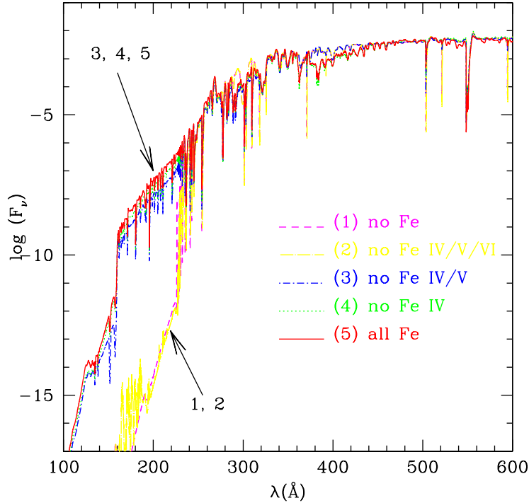
Figure 4.9: Effect of the addition of different Fe ions on the extreme UV spectral energy distribution of a typical O star with T_{\text{eff}} = 41783 K, \log g = 4.02 , \dot{M} = 6.76 \cdot 10^{-7} M_{\odot} \text{ yr}^{-1} and v_{\infty} = 2690 \text{ km s}^{-1} . The details of the models are given in Table 4.1.
