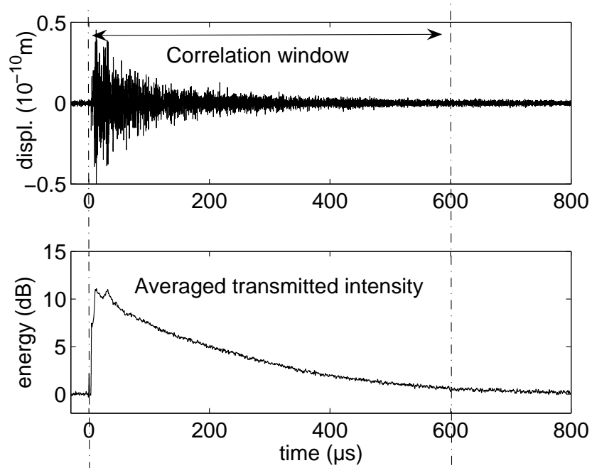
FIG. 5.16 – Top : typical waveform obtained through the scattering slab around 1 MHz. The sensitivity of the heterodyne interferometer is 10^{-4} \text{Å} / \sqrt{\text{Hz}} corresponding the optimal level of optical reflection on the sensed surface. After averaging over 100 records we reached the precision of 10^{-2} \text{Å} . Bottom : intensity averaged over several source/sensor positions.
