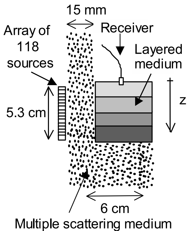
FIG. 6.1 – Experimental setup.
