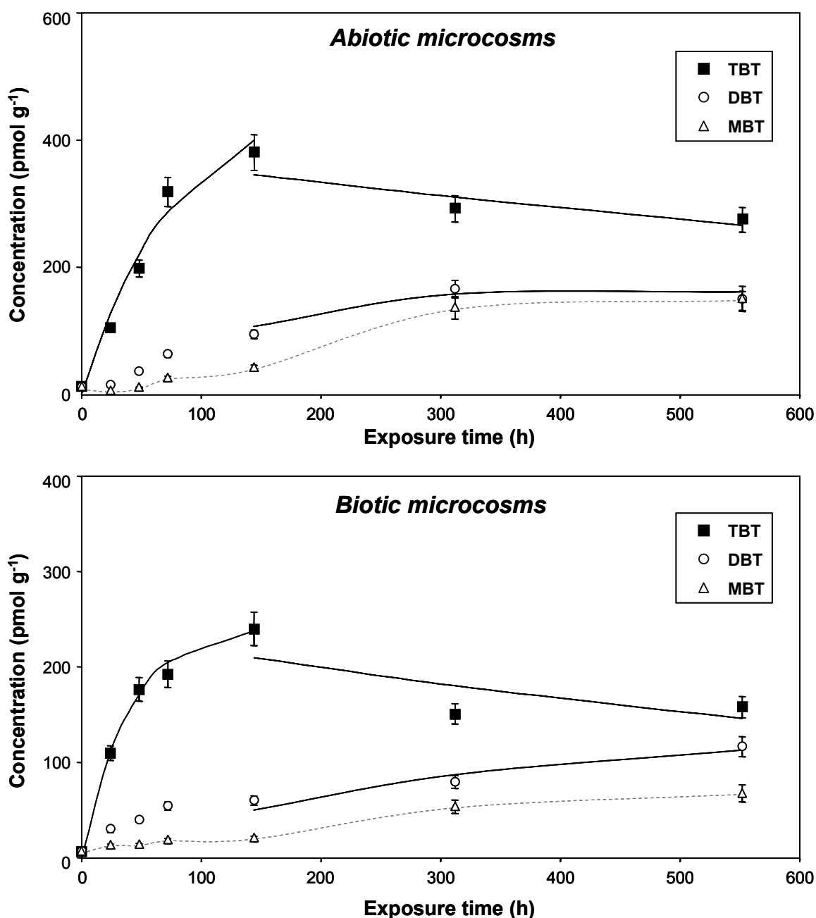
Figure 3 —Experimental and predicted (solid lines) distribution of butyltin concentrations in sediments of the abiotic and biotic microcosms. Errors bars represent the mean deviation obtained from duplicate microcosms
