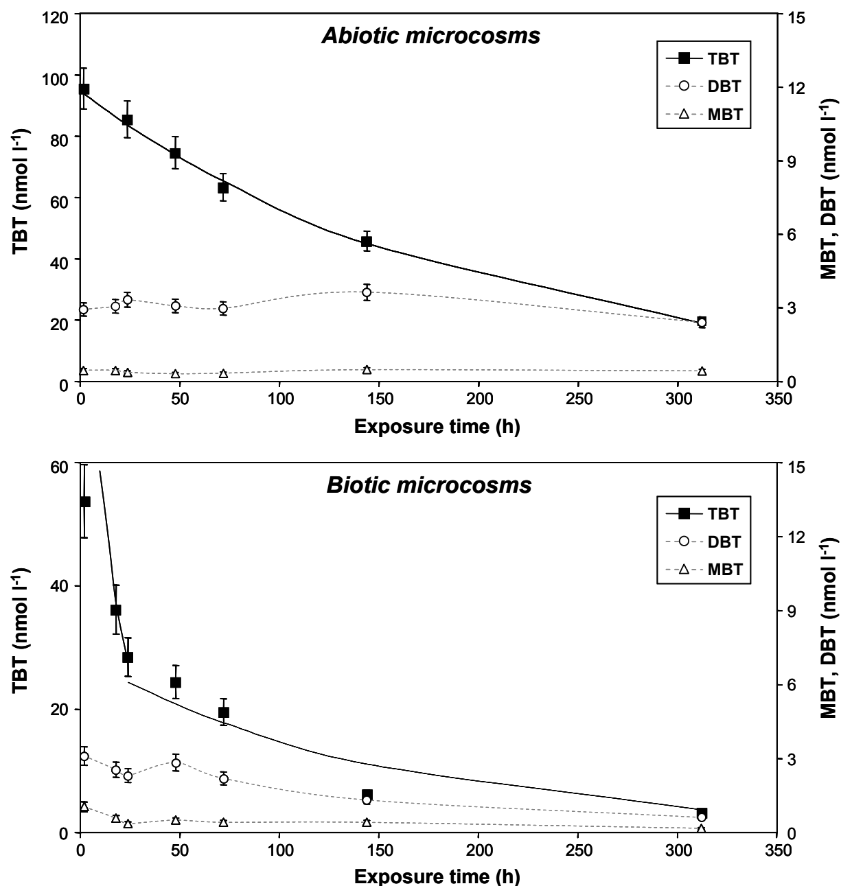
Figure 2 –Experimental and predicted (solid lines) distribution of butyltin concentrations in filtered waters of the abiotic and biotic microcosms. Errors bars represent the mean deviation obtained from duplicate microcosms
