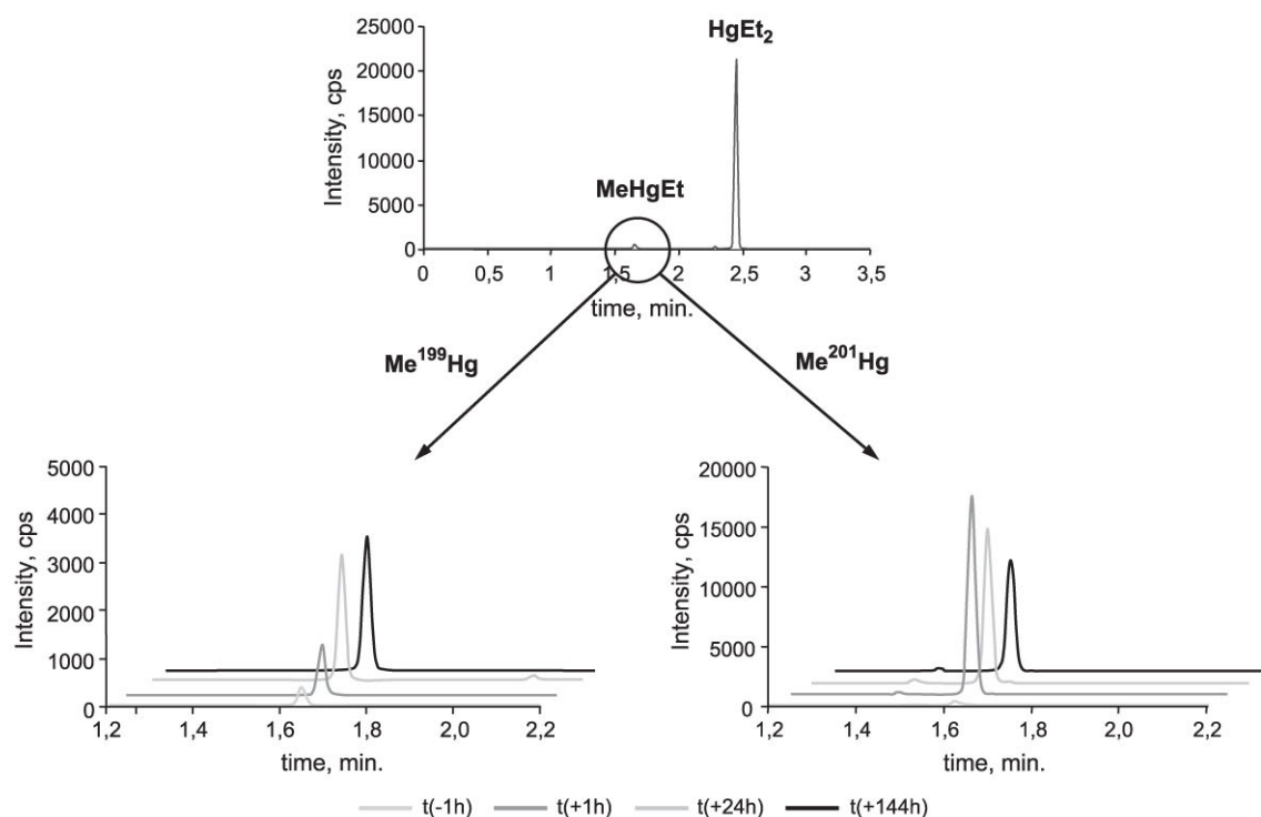
Fig. 3. Chromatograms obtained for the \text{MM}^{199}\text{Hg} and \text{MM}^{201}\text{Hg} evolution under anaerobic nonsterile incubation conditions. The chromatograms at different incubation times are shifted for clarity. t(-1) : 1 h before enriched species spike; t(+1) , (+24) and (+144) : 1, 24 and 144 h, respectively, after the enriched species spike.
