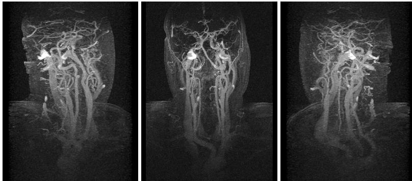
Figure 9: Maximum Intensity Projections (MIP) of a typical blood pool angiography data set, showing the vessels of the head and neck. Three MIPs are presented, with varying angles around the y (head to feet) axis: -45^\circ , 0^\circ and 45^\circ .
